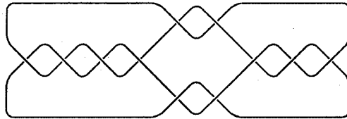
FIGURE 2. Goeritz's unknot
