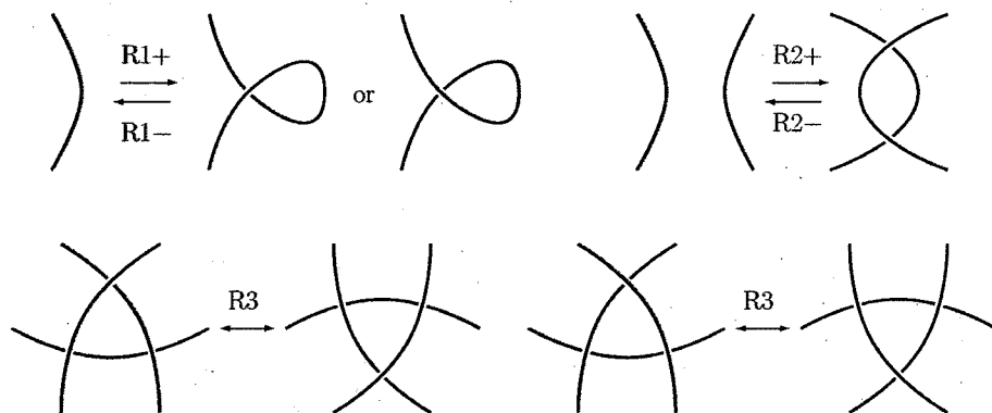
FIGURE 1. Reidemeister moves
