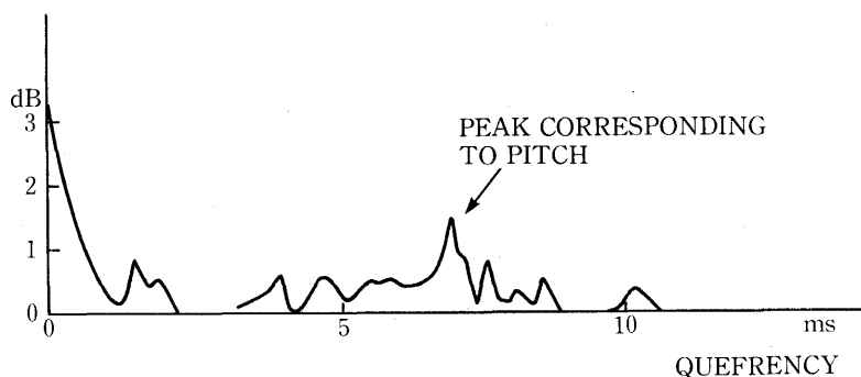
(a) Cepstrum in a voiced interval (noise free)
