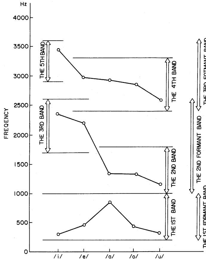
Fig. 4.1. Formant frequency of five vowels and formant bands
