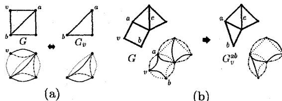
Figure 2: (a) An example of a minimal 0-graph G such that G_v^{ab} is not a minimal 0-graph for d = 2 and D = 3 . Notice that G_v is a 0-graph and hence G_v^{ab} is not minimal. (b) An example of a minimal 0-graph G such that G_v^{ab} is not minimal and also G_v is not a 0-graph for d = 2 and D = 3 . Notice that there exist 3 edge-disjoint spanning trees in \tilde{G}_v^{ab} that contain no edge of \tilde{e} .
