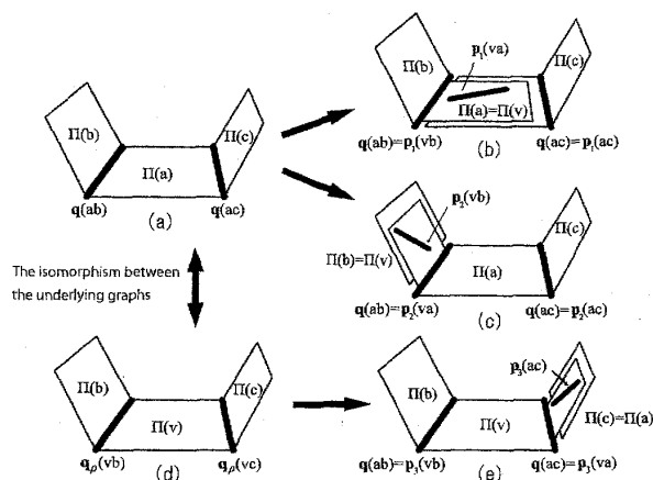
Figure 3: The realizations given in the proof of Lemma 6.7 around v , where the hyperplanes associated with the vertices other than v, a, b, c are omitted. (a) (G_v^{ab}, \mathbf{q}) , (b) (G, \mathbf{p}_1) , (c) (G, \mathbf{p}_2) , (d) (G_a^{vc}, \mathbf{q}_\rho) and (e) (G, \mathbf{p}_3) .
