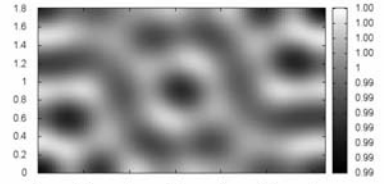
図2: a = 8, b = 49, c = 1, d = 1/32, \mu = 1, l = 2 の t = 500 における計算結果
