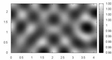
図 6: a = 8, b = 32, c = 1, d = 1/16, \mu = 1, l = 4\sqrt{7} の t = 500 における計算結果
