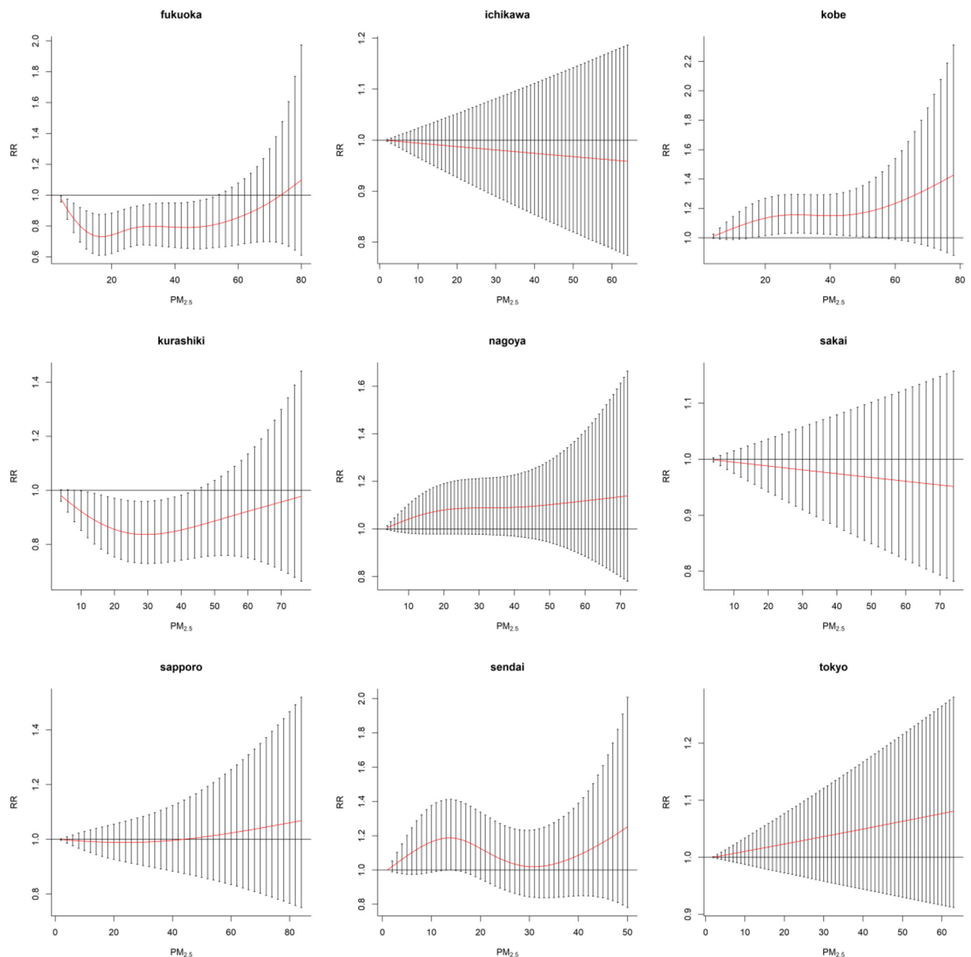
Fig. 2. First stage, city-specific GAM risk curves of the nine Japanese cities.
