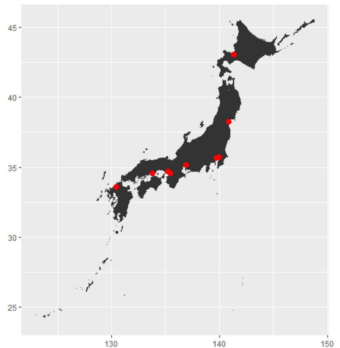
Fig. 1. Geographical location of the nine cities across Japan.
