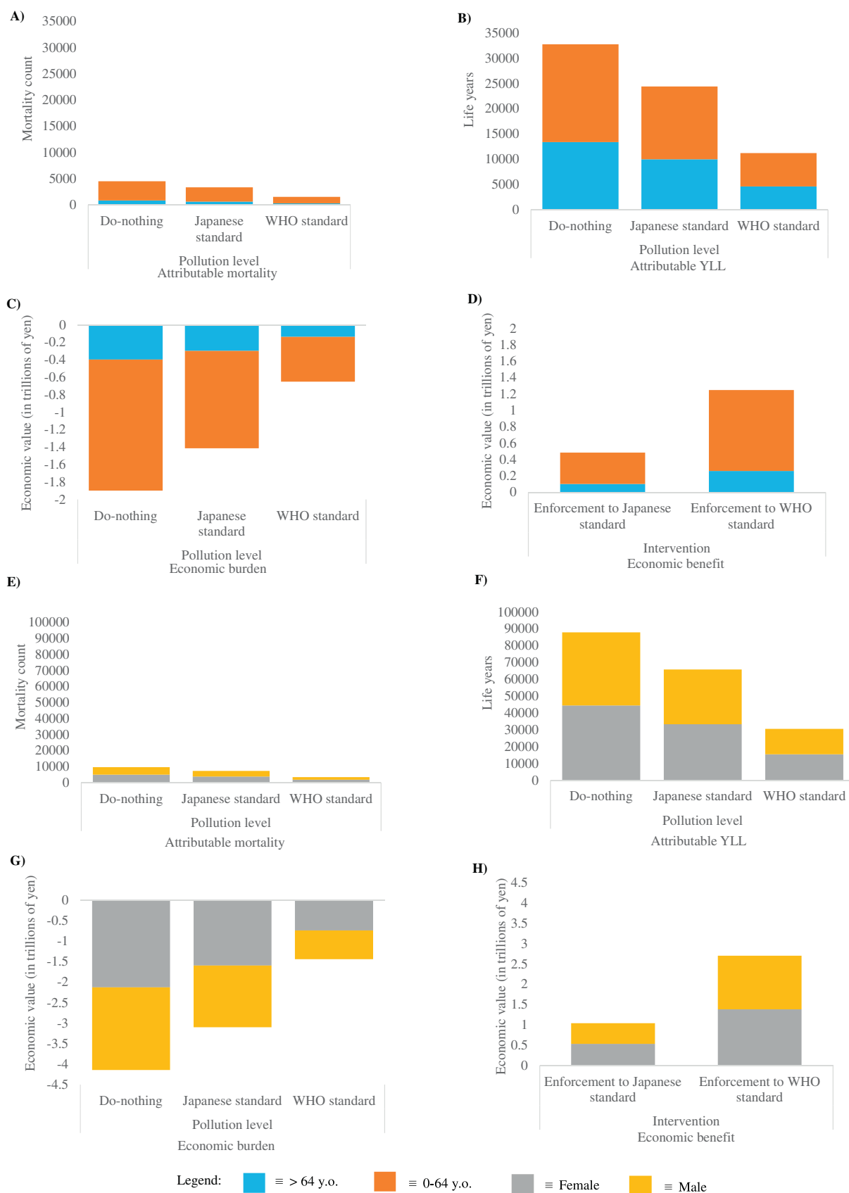
Fig. 5. Health impact of air pollution on age- and sex-specific mortality through the different HIA metrics.
