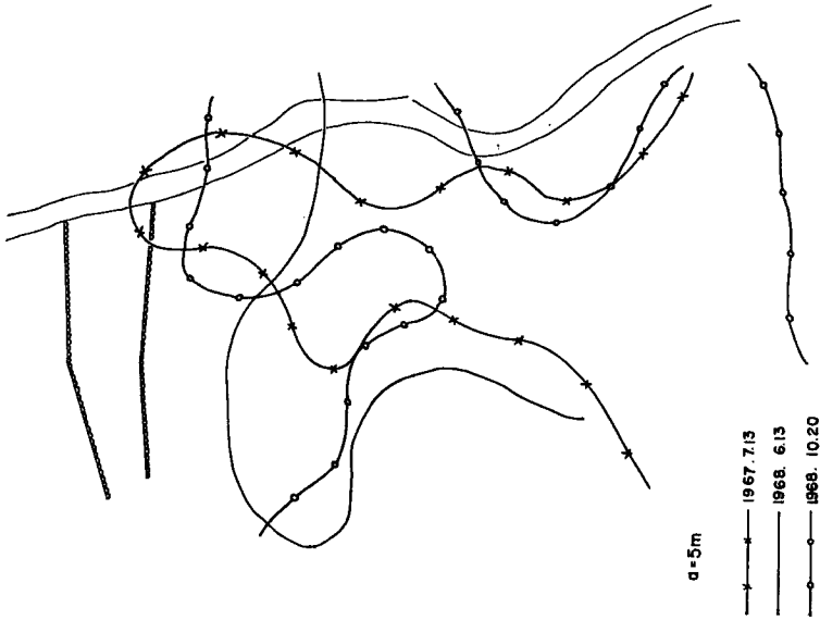
Fig. 13 The variation of the location of the lowest apparent resistivity value during about 15 months at a=5m , Kushibayashi landslide area
