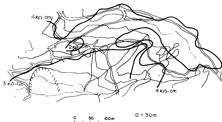
Fig. 3 The distribution map of an apparent resistivity value at a=30\text{m} , Tanokura landslide area
