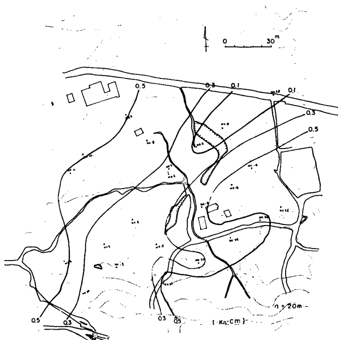
Fig. 10 The distribution map of an apparent resistivity value at a=20\text{m} , Mikage landslide area
