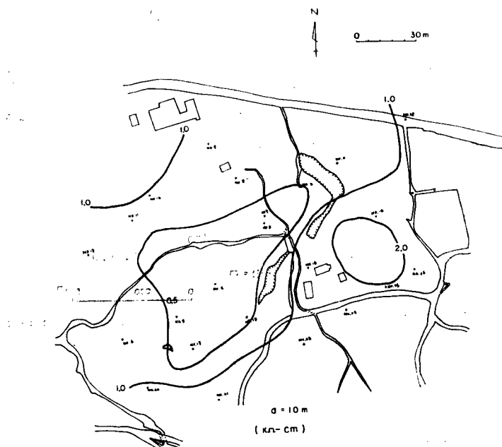
Fig. 9 The distribution map of an apparent resistivity value at a=10\text{m} , Mikage landslide area
