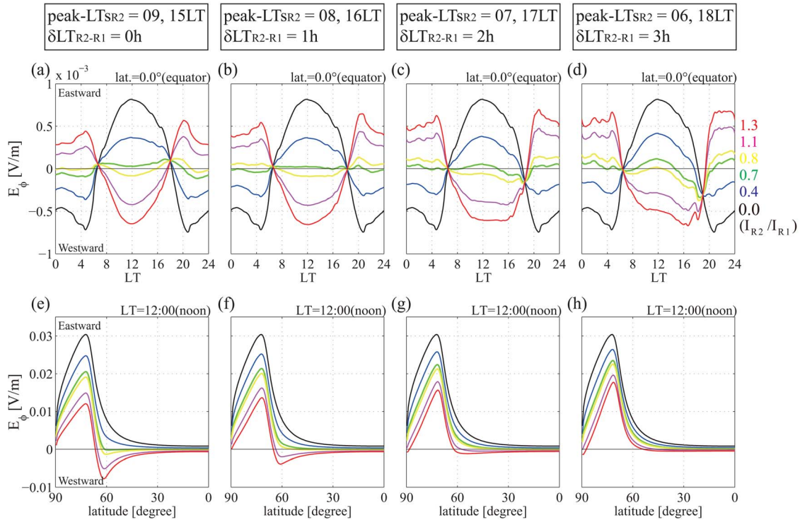
Figure 6. (a–d) Local time profiles of the longitudinal electric field component, E_\phi , along the equator and (e–h) latitudinal profiles along the noon meridian. Formats are the same as in Figure 3; E_\phi is positive eastward. Horizontal axis ranges from 00:00LT to 24:00LT (Figures 6a–6d) and from the north pole (90.0°) to the equator (0.0°) (Figures 6e–6h). Black, blue, green, yellow, magenta, and red colors represent the cases with I_{R2}/I_{R1} of 0.0, 0.4, 0.7, 0.8, 1.1, and 1.3. From left to right, peak-LTSR2 (the peak local times of R2-FAC) are moved toward the nightside from 09:00 and 15:00 (equals to that of R1-FAC, the same as in Figure 3) to 06:00 and 18:00 (purely dawn and dusk) with an increment of one hour, as the same as Figure 5.
