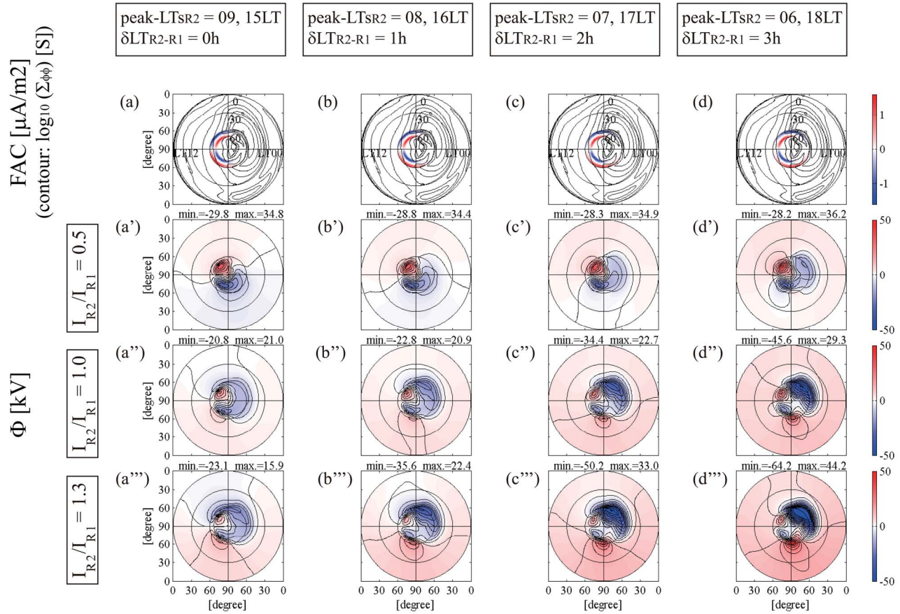
Figure 5. Potential pattern variations with I_{R2}/I_{R1} and peak- LT_{SR2} (the peak local times of R2-FAC). Each panel is displayed in the same format as Figure 2. From left to right, the peak local times of R2-FAC are moved toward the nightside from 09:00 and 15:00 (equals to that of R1-FAC, the same as in section 3.2) to 06:00 and 18:00 (purely dawn and dusk) with an increment of one hour. (a–d) The FAC distributions with I_{R2}/I_{R1} of 1.3 are shown for the purpose of reference. Shown are the results with I_{R2}/I_{R1} of (a'–d') 0.5, (a''–d'') 1.0, and (a'''–d''') 1.3.
