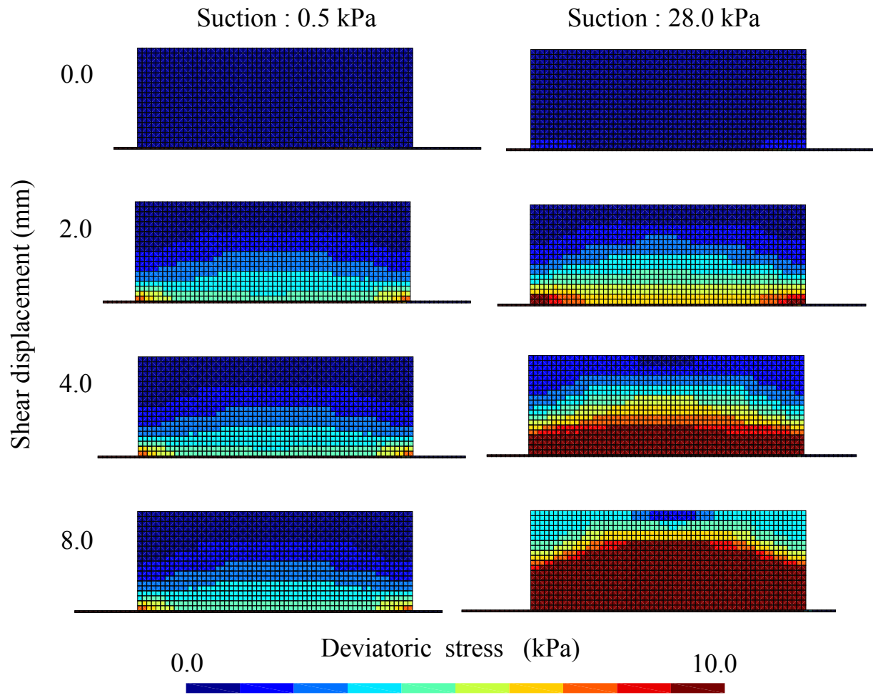
Figure 6.5: Contour map of deviatoric stress of soil and root domains. Shear stress of soil domain increases with the increase of suction.
