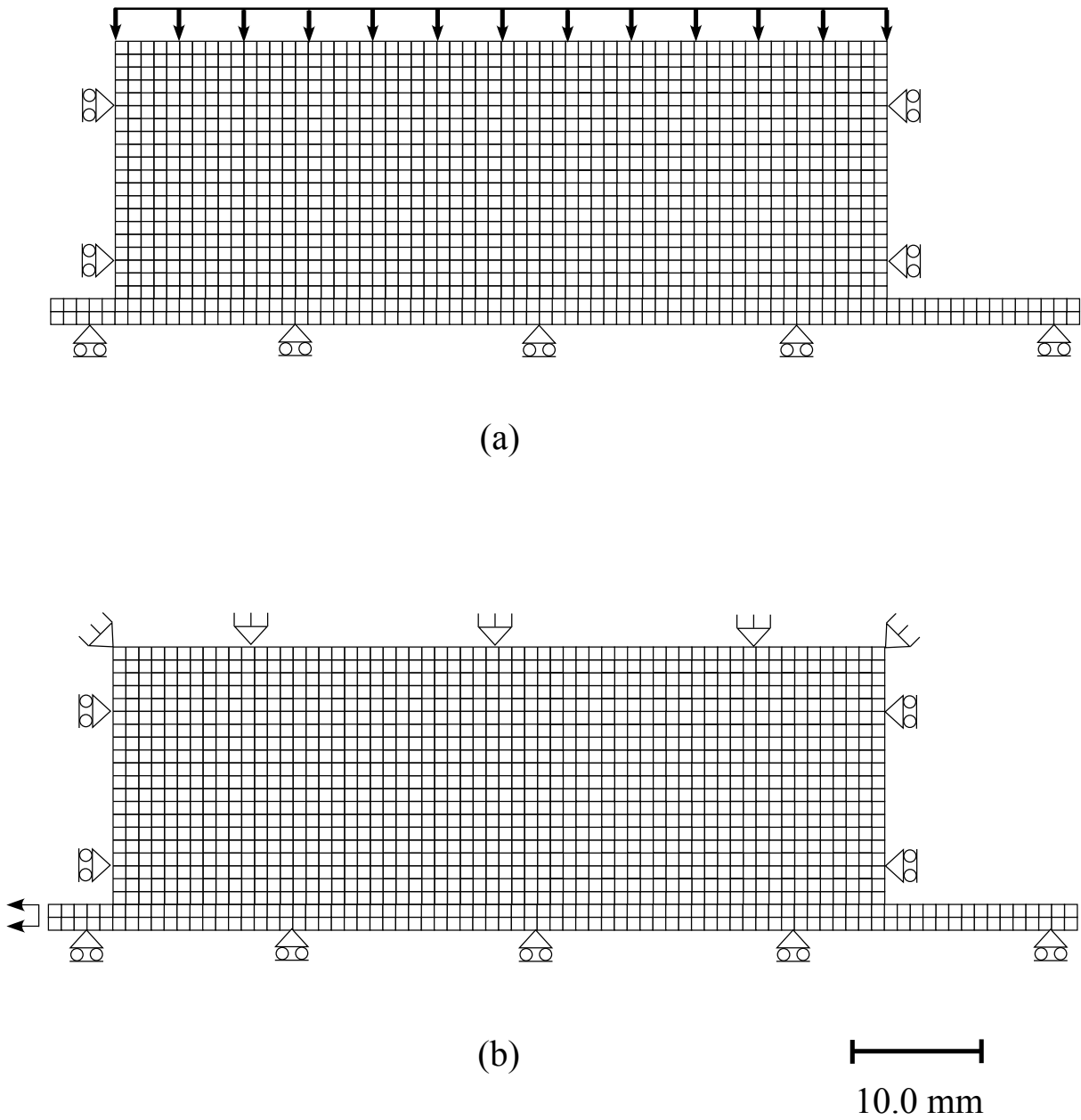
Figure 4.12: Mesh and boundary conditions of pullout tests: (a) prior to simulation, initial stress is loaded to reproduce experimental conditions. (b) The topsoil is vertically fixed during the pullout simulation.
