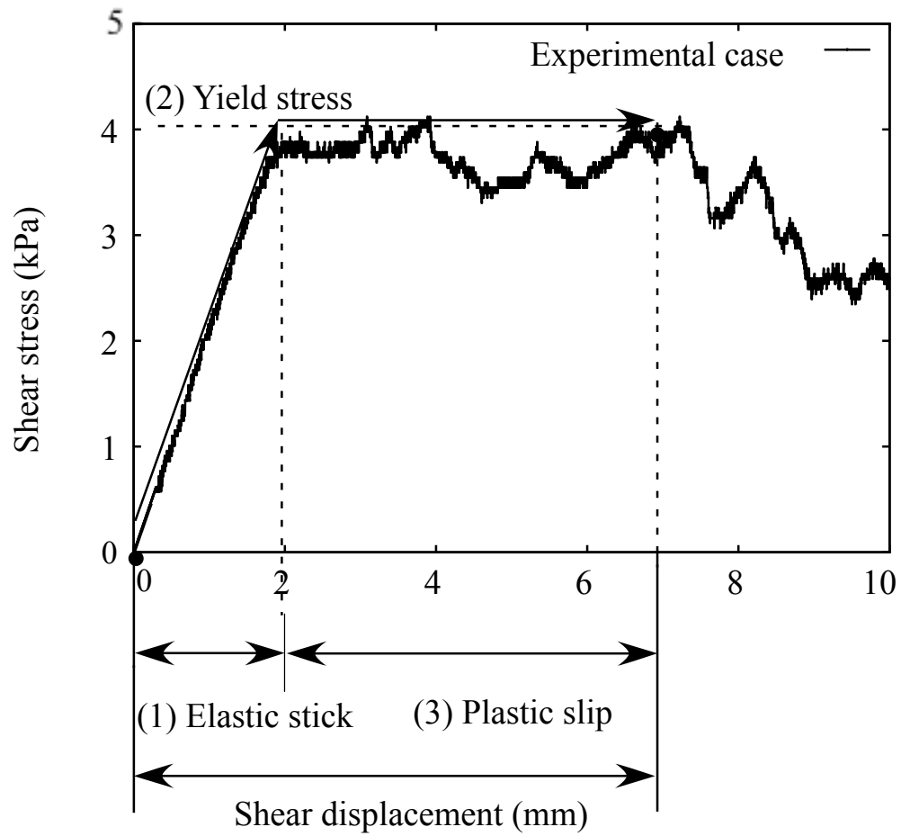
Figure 3.14: Additive decomposition of displacement and shear stress vs. displacement by elastio-perfectly-plastic model.
