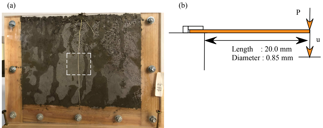
Figure 4.10: Schematics of bending test to measure Young's modulus of a root: (a) Image of soil-box and root used in bending test and (b) Schematic of bending test and properties of root segment.
