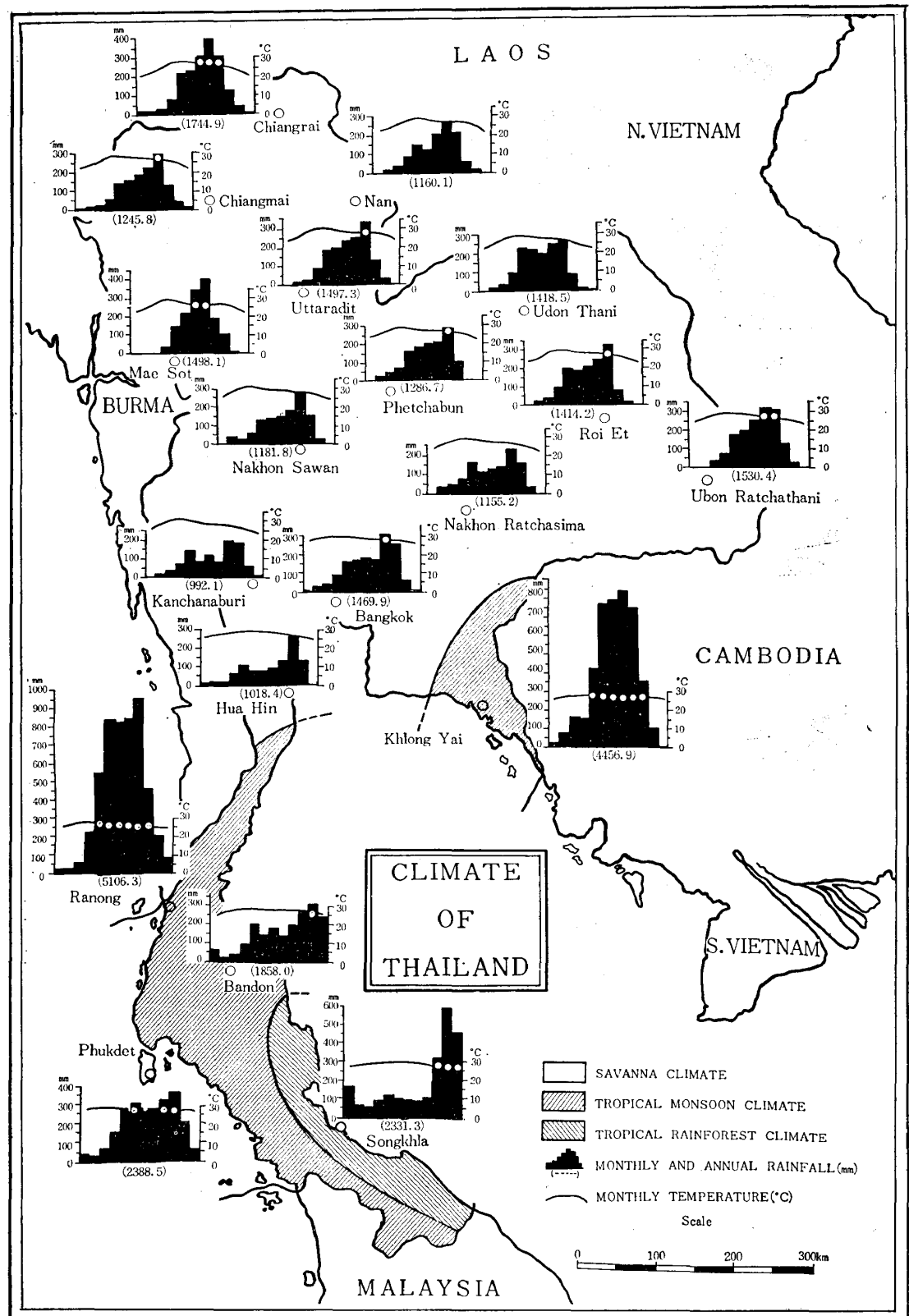
図-5 Climate of Thailand
