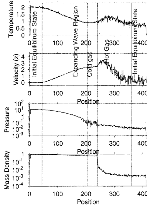
FIG. 4: Spatial profiles of temperature, velocity ( z ), pressure, and mass density at t = 15 : System size is taken to be L_x = 32, L_y = 32, L_z = 408 and size of magma chamber is 32 \times 32 \times 200 . Initial mass density and temperature are taken to be 1 and 2, respectively. We can recognize characteristic regions. From right, “initial equilibrium state”, “hot gas region”, “cold gas region”, “expanding wave region”, and “initial equilibrium state” again are observed. These regions are indicated by gray rectangular.
