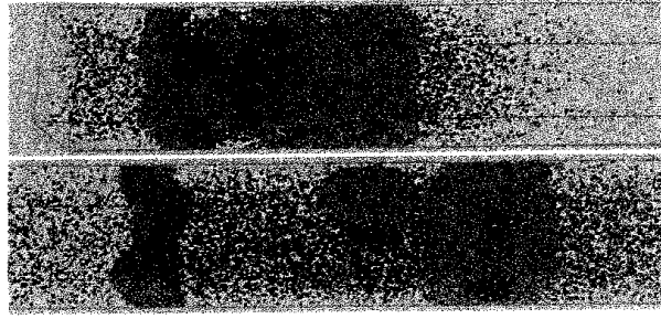
FIG. 3: Snapshots of simulation: (Up) Snapshot at t = 40 . (Down) Snapshot at t = 170 . Parameters are identical to ones of Fig. 2. Eruption propagates to the right direction. Only particles originated from the chamber are plotted; A red ball represents a magma particle, and blue one is a gas particle. At the initial condition t = 0 , blue and red particles are uniformly mixed in the chamber.
