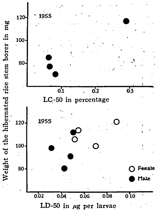
Fig. 2. Relation between LC-50 or LD-50 and the average weight of the hibernated rice stem borer reared on different varieties of rice plant and applied with parathion and methyl parathion.
