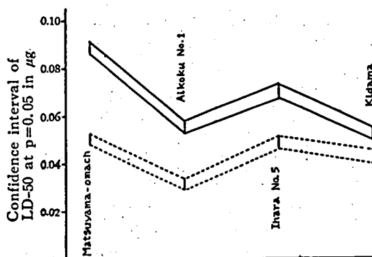
Fig. 1. Variation in the resistance to methyl parathion of the hibernated rice stem borer reared on different varieties of rice plant. Solid lines cover the confidence interval of LD-50 at p=0.05 of the female and broken lines that of the male.
