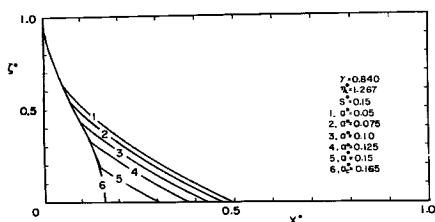
Fig. 5 Theoretical figure of interface by pumping salt water
