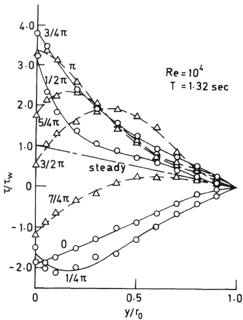
Fig. 4.11. Shear stress profiles in pulsating flow ( T < T_c ).
