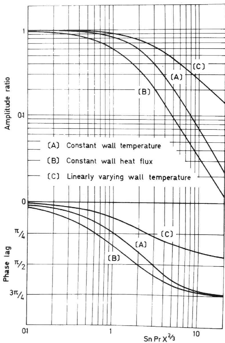
Fig. 3.2. Bode diagram of local Nusselt number for three heating conditions.
