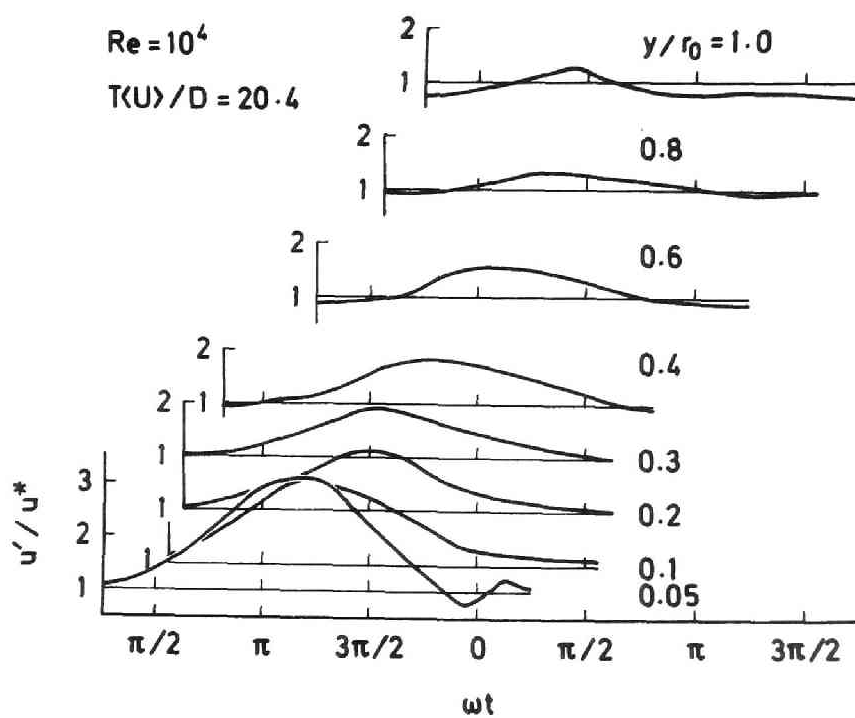
Fig. 5.11. Variations of turbulence intensity after rapid change of time scale.
