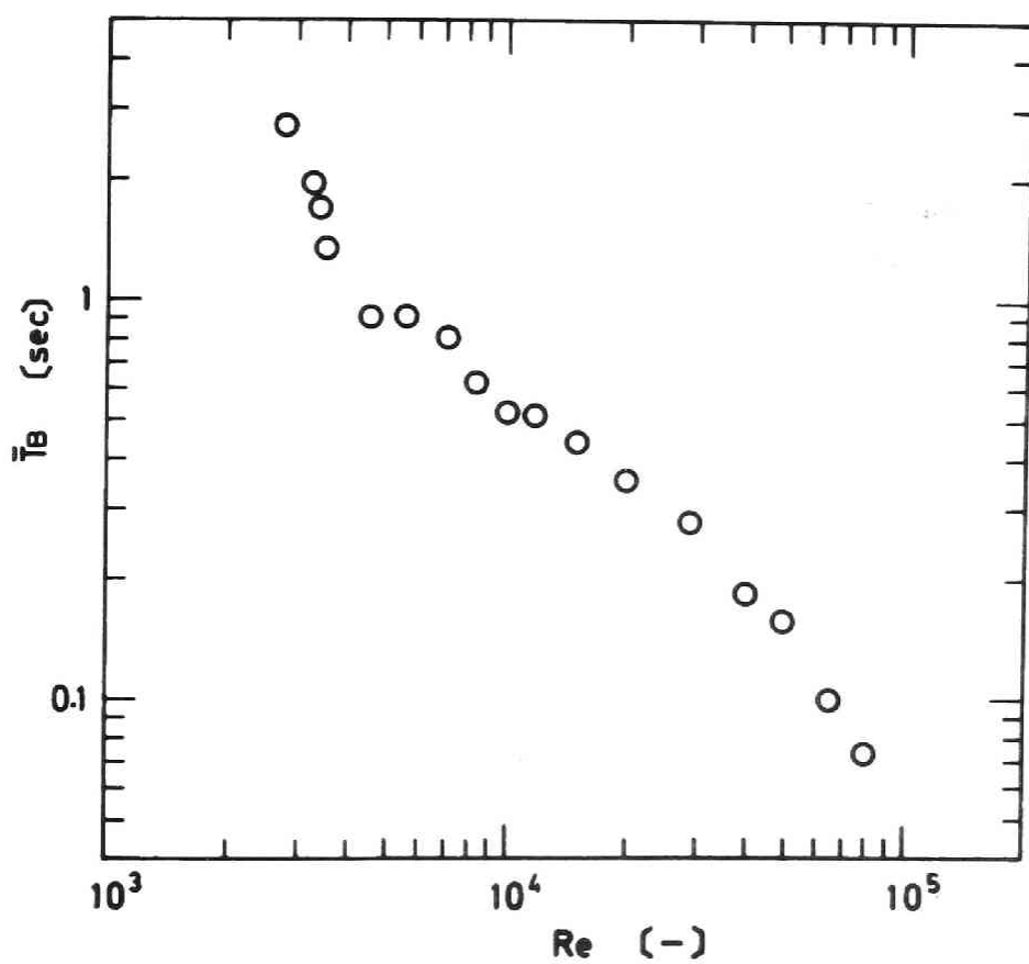
Fig. 4.18. \overline{T}_B as a function of Reynolds number.
