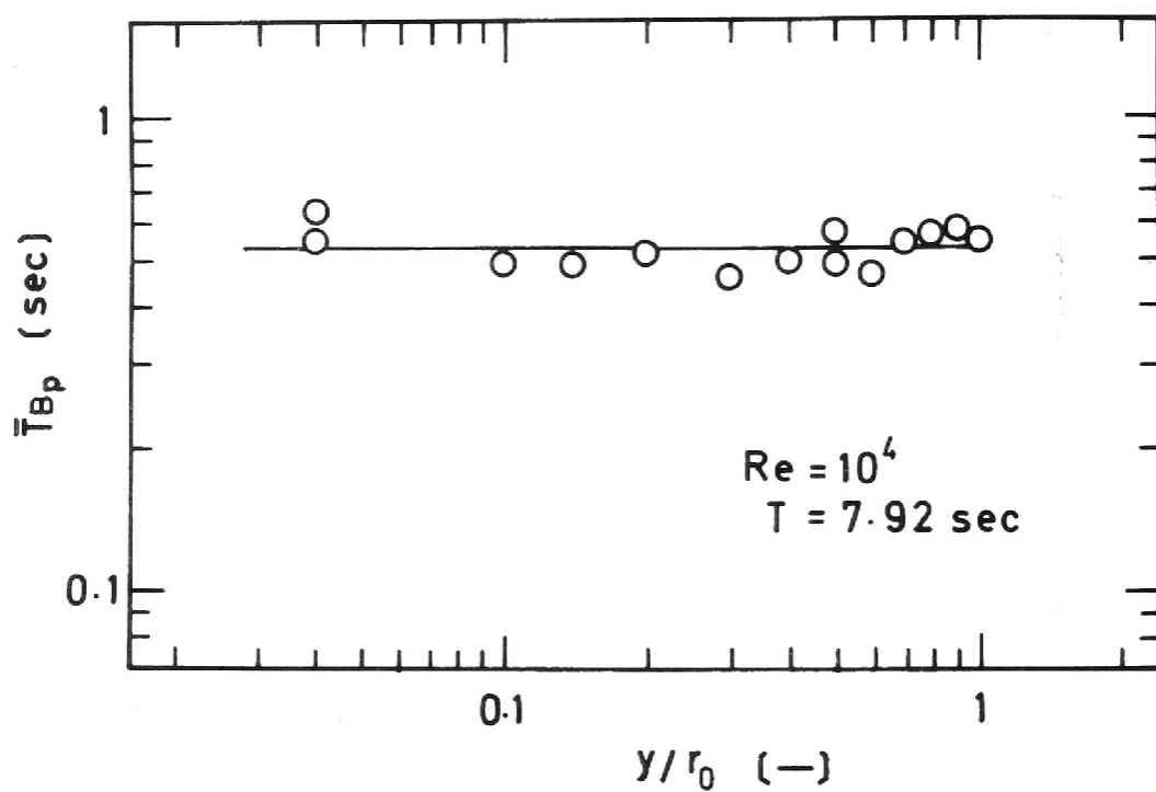
Fig. 4.20. Radial distribution of \bar{T}_B in pulsating flow.
