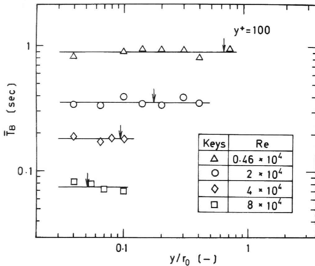
Fig. 4.17. Radial distribution of \bar{T}_B .
