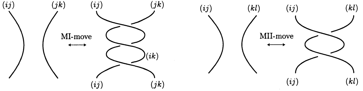
Figure 2: MI, II moves of labeled diagrams
