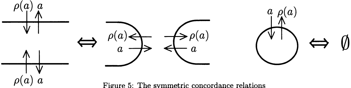
Figure 5: The symmetric concordance relations
