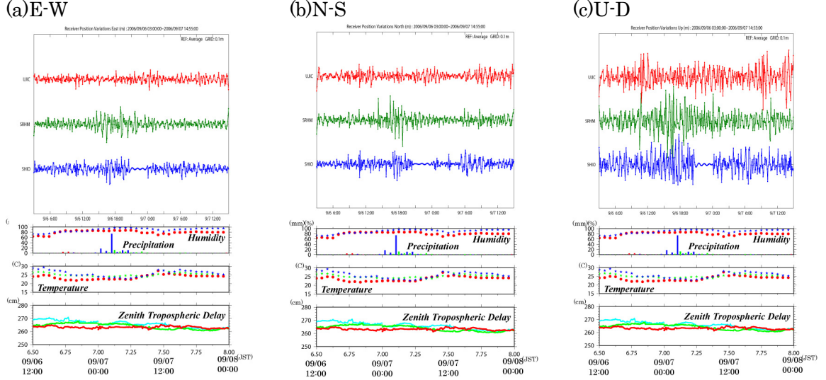
Fig.4. The kinematic GPS results of three observation points, Uji, Shirahama, and Shionomisaki, on September 5-8, 2006. The graph is (a) East-West, (b) North-South, and (c) Up-Down component, respectively. Three lower graphs show the Humidity, Precipitation, Temperature, and Zenith tropospheric delay. Only the record of Shirahama is large at the time of the front passage, and positioning accuracy decreases more.
