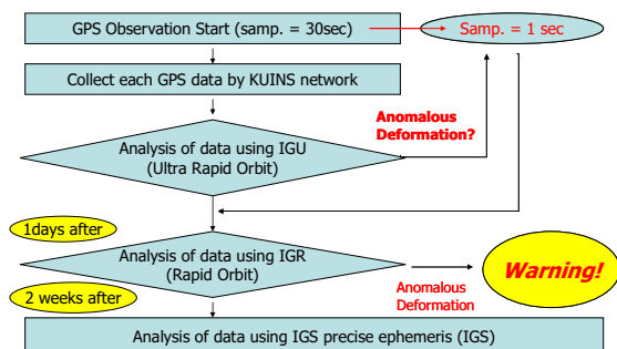
Fig.5. The flow chart of a semi-real time monitoring system.
