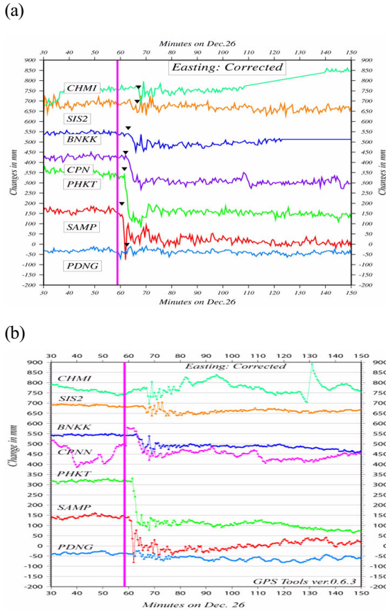
Fig.3. Comparison of kinematic GPS analysis of the 2004 Sumatra-Andaman Earthquake. Upper graph shows the analysis by the GIPSY software [Hashimoto et al., 2006]. Lower graph (b) shows by the GPS-Tools software in this study.
