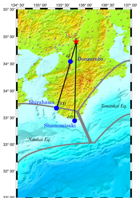
Fig.1. Baseline Map of this experiment. Number of Circles is Baseline length from Uji (km).
