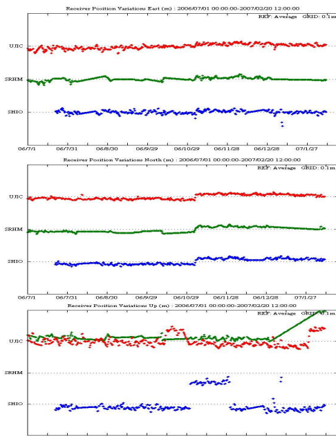
Fig.2. Static analysis result of the continuous observation point established by DPRI, Kyoto University. These graphs show the East-West, North-South, and Up-Down component, respectively. The step seen in the beginning in November is the change of the International Terrestrial Reference Frame (ITRF2000 to ITRF2005).
