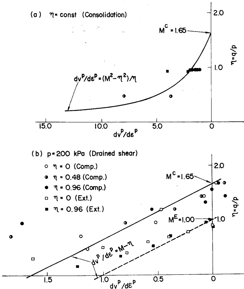
Fig. 5. Correlations between the plastic strain increment ratio dv^P/d\epsilon^P and the stress ratio \eta = q/p .
