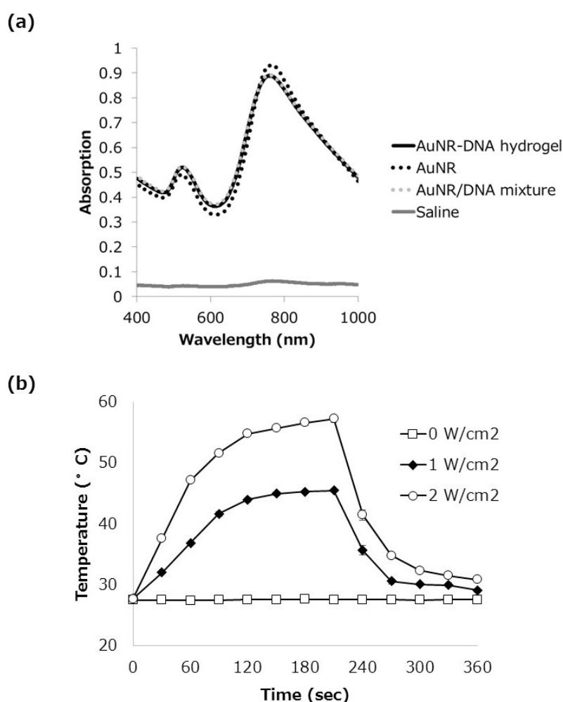
Figure 21 : Optical/Photothermal Properties of AuNR-hydrogel. (a) UV-visible absorbance spectra of AuNR-DNA nanocomposites and their components. UV-visible spectra of Saline, Hydrogel(cg), AuNR, AuNR-ODN/hPODNA(cg), and AuNR-hydrogel(cg) were recorded using NanoDrop 2000 spectrophotometer. (b) Photothermal behavior of the AuNR-DNA nanocomposites in response to laser irradiation at wavelength of 780 nm. The temperature was monitored using contact thermometer.
