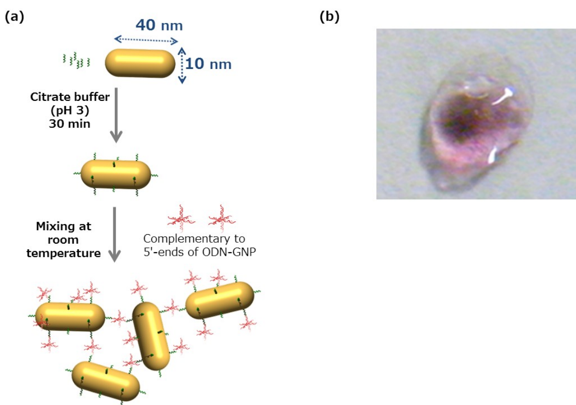
Figure 20 : Appearance of AuNR-hydrogel. (a) Schematic illustration of synthesis of AuNR-hydrogel(cg). DNA with polyadenine sequence was adsorbed onto gold nanorods in citrate-buffer with pH 3, in same manner as AuNPs. Hexapodna was prepared by mixing equimolar six ODNs. After preparing each building blocks separately, the two components were mixed at room temperature. (b) Optical image of AuNR-hydrogel(cg).
