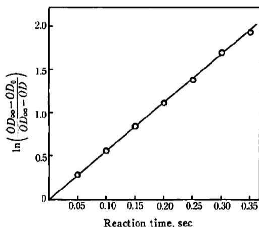
Fig. 5 Pseudo-first order plot of optical density at 443 m\mu in BQ-EtO ^- system at 20°C
