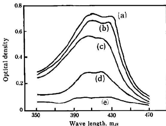
Fig. 1 The change of electronic spectra with time in BQ-EtO - system [BQ] 0 = 1.0 × 10 -2 (mole/l), [EtO - ] 0 = 1.0 × 10 -3 (mole/l), reaction time (sec); (a) 45 (b) 70 (c) 120 (d) 240 (e) 600
