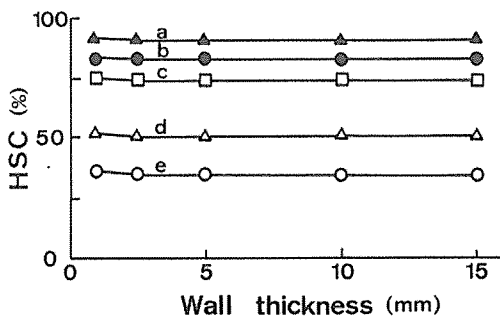
Fig. 5 Change in HSC with wood wall thickness at various WA/RV ratio. Temp. change: 6.0\text{--}12.4^\circ\text{C} WA/RV [\text{m}^2/\text{m}^3] : a: 4.2, b: 2.1, c: 1.3, d: 0.6, e: 0.3
