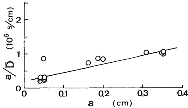
Fig. 2 Relationship of a/\bar{D} vs. a to determine S value. Temp.: 20^{\circ}\text{C}
