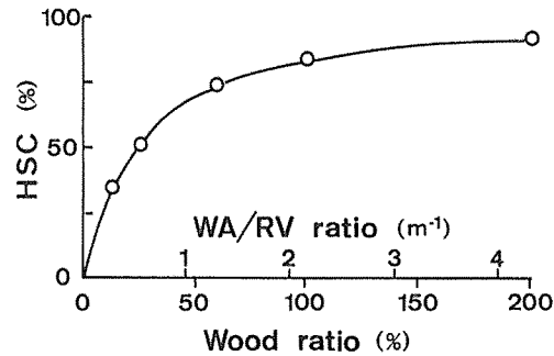
Fig. 4 Change in humidistat coefficient ( HSC ) with wood ratio (per inner surface area of room) and wood surface area per room volume ( WA/RV ). Room size = 3.6\text{m} \times 2.7\text{m} \times 2.4\text{m} , wood thickness = 1.2\text{cm}
