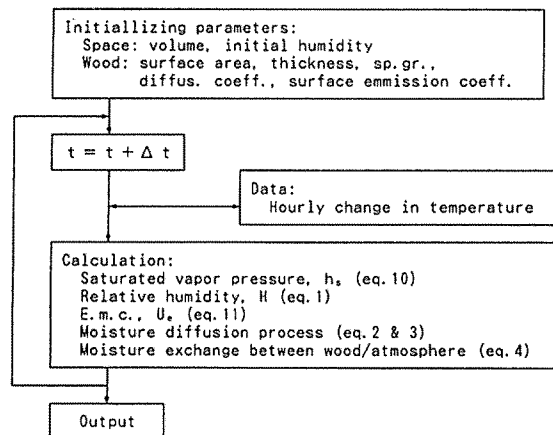
Fig. 1 Flow-chart for simulation of humidity control by wood.
