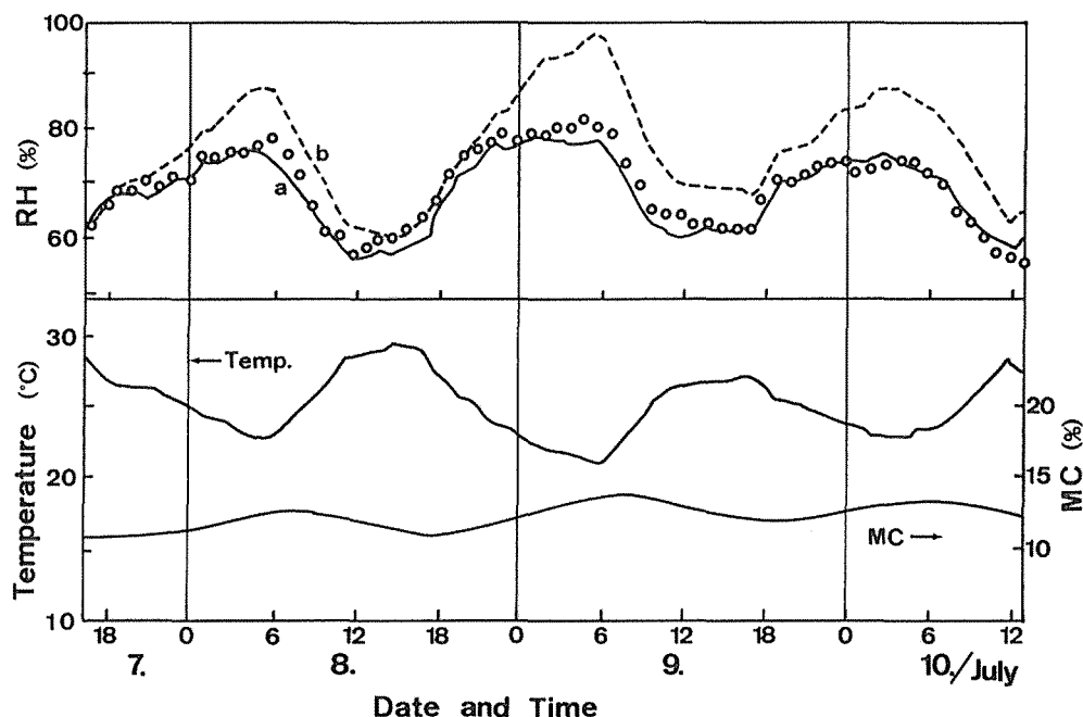
Fig. 3 An example of relative humidity change in closed spaces with and without wood.
