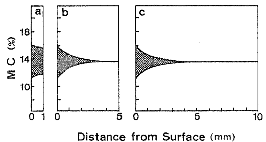
Fig. 6 Range of moisture content oscillation in wood wall. Temp. change: 6.0\text{--}12.4^\circ\text{C} Wall thickness: a: 1\text{mm} , b: 5\text{mm} , c: 10\text{mm}
