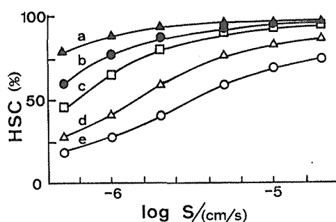
Fig. 7 Change in HSC with surface emission coefficient S at various WA/RV ratio. Temp. change: 6.0-12.4 °C WA/RV [ m^2/m^3 ]: a: 4.2, b: 2.1, c: 1.3, d: 0.6, e: 0.3
