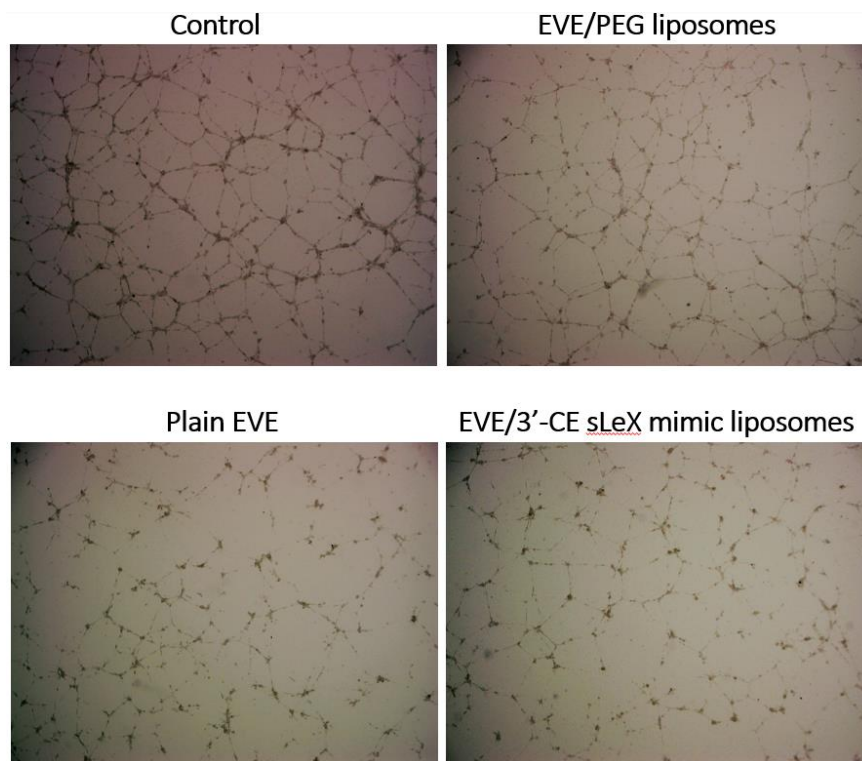
Figure 5. Effect of EVE or EVE-loaded liposomes on tube formation in HUVECs treated with TNF- \alpha and IL-1 \beta . HUVECs were plated on Matrigel and treated with proinflammatory cytokines for 5 h. The cells were treated with 1 \mu M plain or liposomal EVE for 5 h and observed under a microscope.
