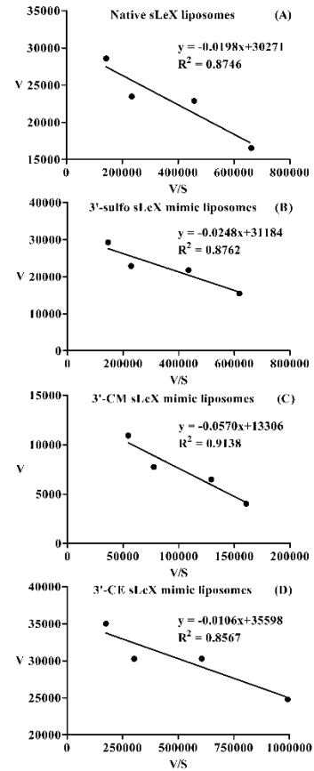
Figure 3. Eadie-Hofstee diagrams of the uptake of (A) native sLeX, (B) 3'-sulfo sLeX mimic, (C) 3'-CM sLeX mimic, and (D) 3'-CE sLeX mimic liposomes in HUVECs pretreated with 100 ng/mL TNF-α and 10 ng/mL IL-1β for 5 h. The ordinate and abscissa represent the uptake rate (v) and the uptake rate divided by liposome concentration (v/s), respectively. The regressed equation, together with its regression coefficient, is shown in each panel,
