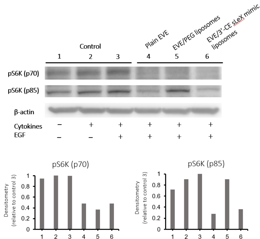
Figure 6. Effect of EVE or EVE-loaded liposomes on phosphorylation of pS6 kinase in HUVECs treated with TNF- \alpha and IL-1 \beta . Following pretreatment with cytokines for 5 h, the cells were incubated with 1 \mu M plain or liposomal EVE for 4 h. The cells were treated with 50 ng/mL hEGF for the last 15 min, lysed with RIPA buffer, and subjected to western blotting using antiphospho- p70 S6 kinase antibody.
