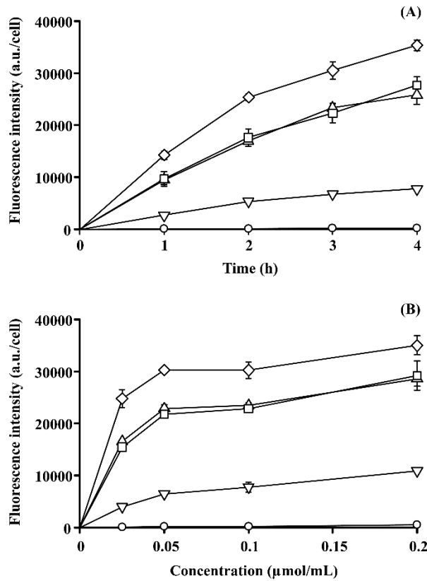
Figure 2. Time-course analyses (A) and concentration dependence (B) of the uptake of fluorescein-labeled liposomes in HUVECs treated with TNF-α and IL-1β for 5 h. Symbols: ○, PEG liposome; △, native sLeX liposome; □, 3'-sulfo sLeX mimic liposome; ▽, 3'-CM sLeX mimic liposome; ◇, 3'-CE sLeX mimic liposome. Results are expressed as mean ± SD of three samples.
