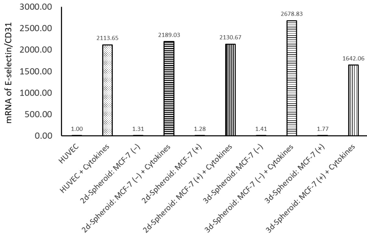
Figure 2. qRT-PCR for E-selectin expression of monolayer cells or spheroids in presence or absence of inflammatory cytokines. (A) mRNA of E-selectin normalized with mRNA of β-actin (B) mRNA of CD31, endothelial cells marker, normalized with mRNA of β-actin (C) mRNA of E-selectin/CD31, indicating E-selectin expressed by HUVECs.
