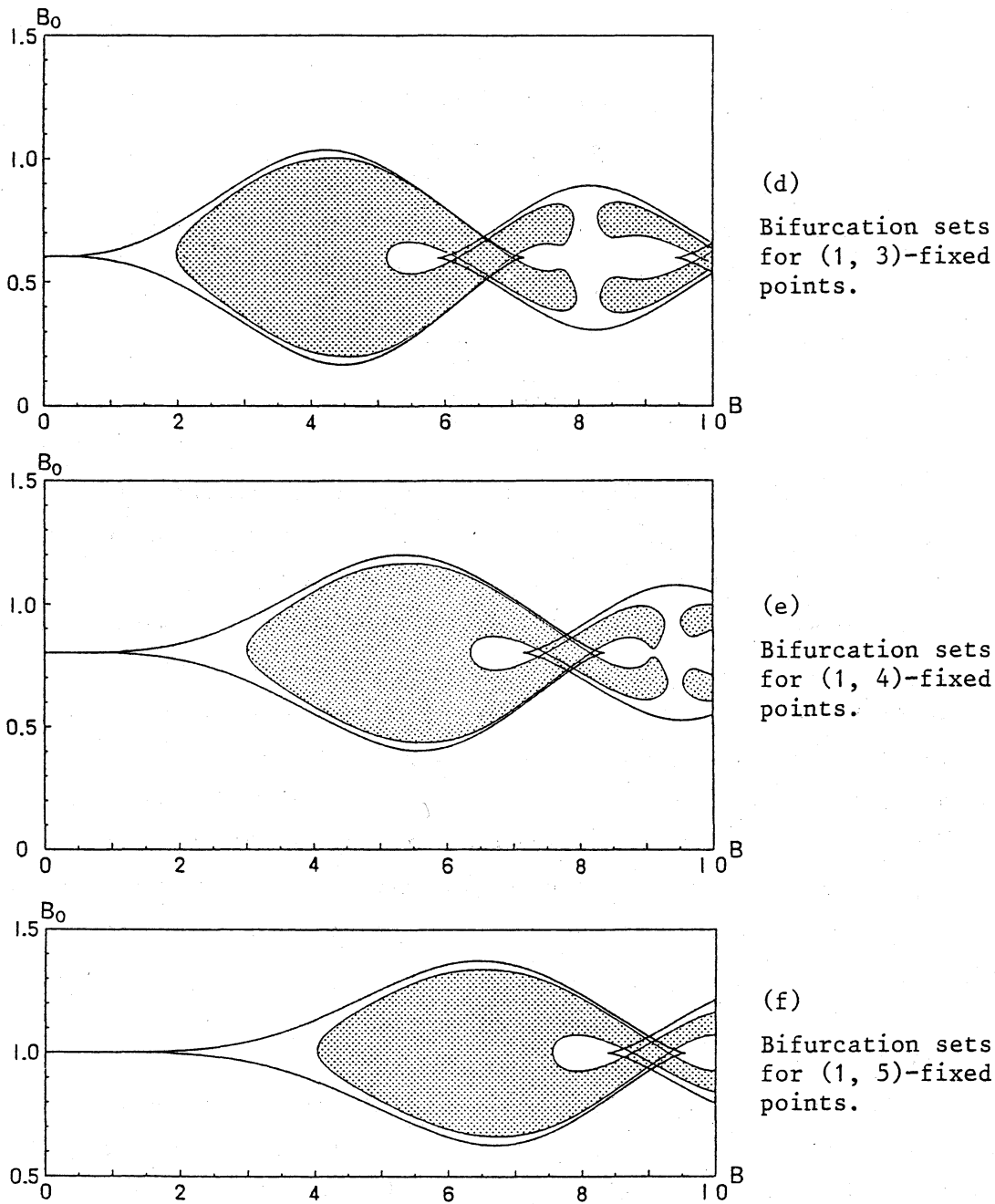
Fig. 5. Bifurcation diagrams for (1, L)-fixed point of T. k = 0.2 , v = 1.0 . Outer boundary curve denotes the set for tangent bifurcation. Boundary curve of shaded portion indicates the set for period doubling bifurcation; see Fig. 1.
