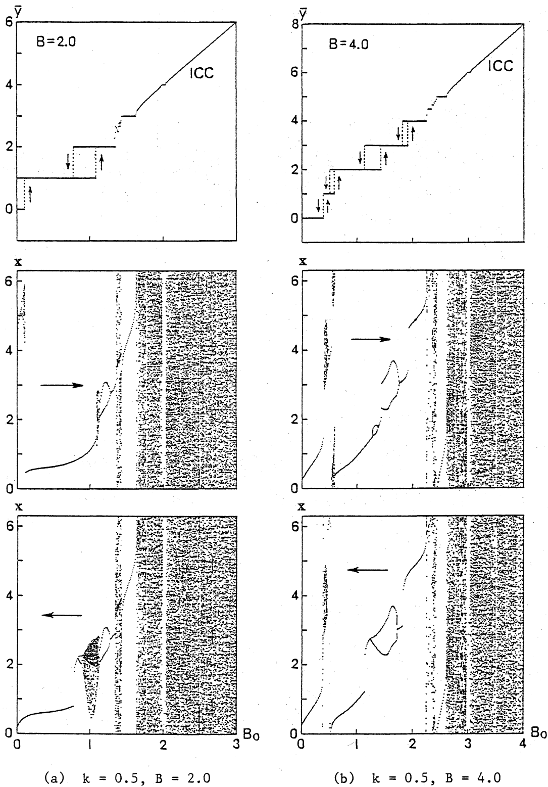
Fig. 4. Phase diagram of x and \bar{y} . The arrow indicates the direction for variation of B_0 .
