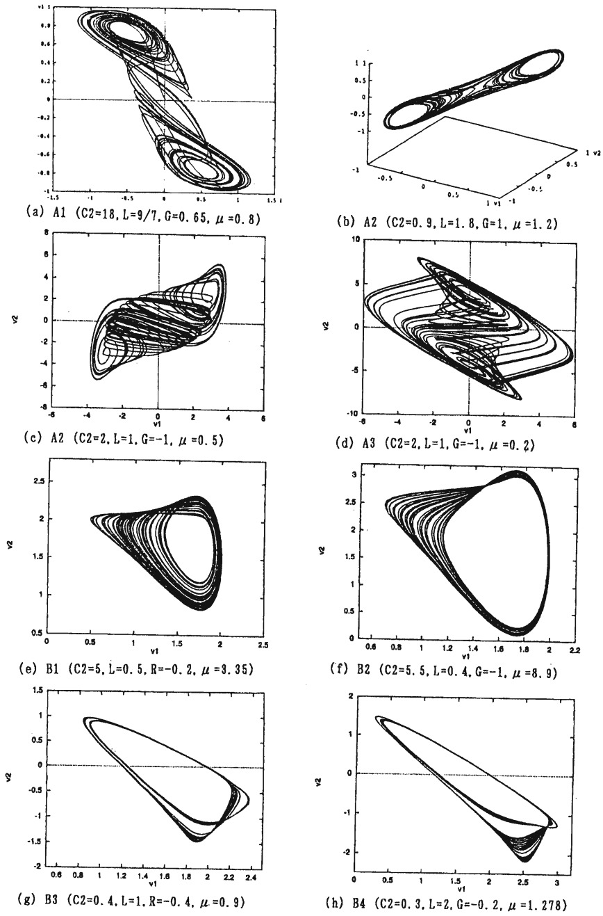
Fig. 6: Some examples of the chaotic attractors ( C_1 = 1.0 ).
