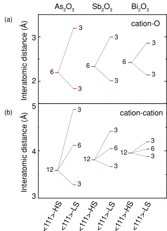
FIG. 5. (Color online) (a) Cation-O and (b) cation-cation interatomic distances in the \langle 111 \rangle -HS and -LS arrangements of the three sesquioxides. The numbers beside the bars show the degeneracy.
