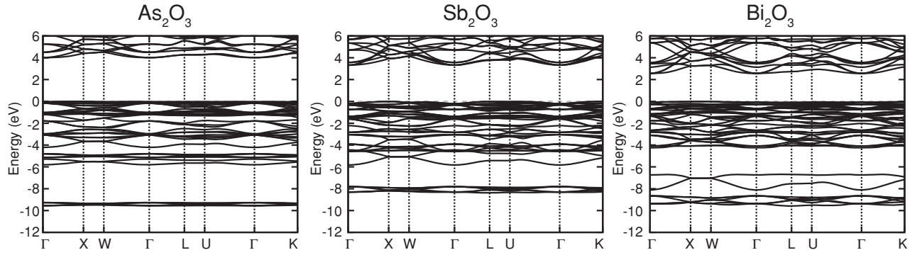
FIG. 6. Electronic band structures of the \langle 111 \rangle -LS arrangements for the three sesquioxides. The top of the valence band is set to 0 on the vertical axis.
