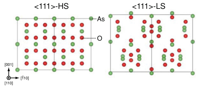
FIG. 4. (Color online) Projection of the \langle 111 \rangle -HS and -LS arrangements of \text{As}_2\text{O}_3 from the [110] direction.
