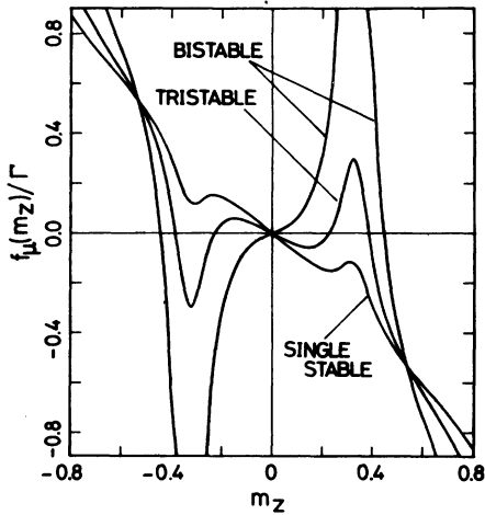
FIG. 3. Plot of the function f_\mu(m_z) for single-stable, tristable, and bistable cases. Parameters are R=0.7 ; 2k_0L = -\pi + 2M\pi ( M : integer); 2\kappa L = 1.5\pi ; and Q_+ = Q_- = 0.1\Gamma (single stable), Q_+ = Q_- = 0.3\Gamma (tristable), Q_+ = Q_- = 1.0\Gamma (bistable). The equilibrium points satisfying f_\mu(m_z)=0 are stable (unstable) when f'_\mu(m_z) < 0 ( > 0 ). In the bistable case, for example, the point m_z=0 is unstable and m_z = \pm 0.44 are stable.
