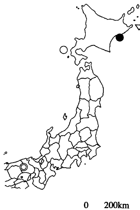
Fig. 9. Distribution of epicenters of M8-class earthquake occurring in and around Japan during the period from 1993 to 1994. ●: Kuroshio-oki Earthquake (M=7.8, Depth=108 km), ○: Hokkaido Nansei-oki Earthquake (M=7.8, Depth=35 km), ▽: Hokkaido Toho-oki Earthquake (M=8.1, Depth=40 km), ◎: Shioya.
