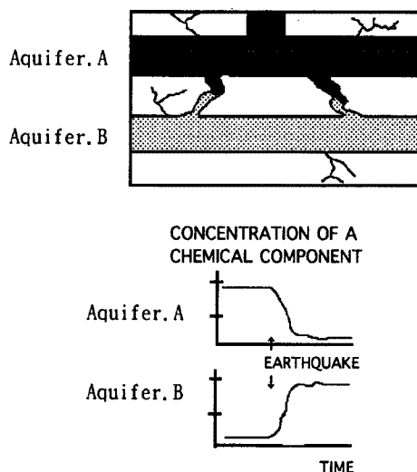
Fig. 1. A Model for change in water quality made by earthquake-caused destruction of the underground structure. Aquifer A: Aquifer where the concentration of a chemical component of the groundwater is high, Aquifer B: Aquifer where the concentration of it is low.
