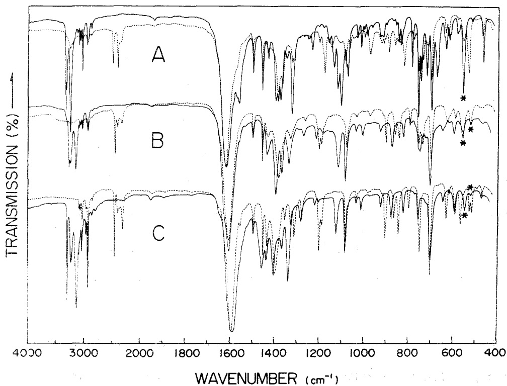
Fig. 2 IR Spectra of \text{Cu}(\text{L-phe})_2 , and \alpha - and \beta - \text{Cu}(\text{DL-phe})_2 , in the Region above 450\text{ cm}^{-1} ,
