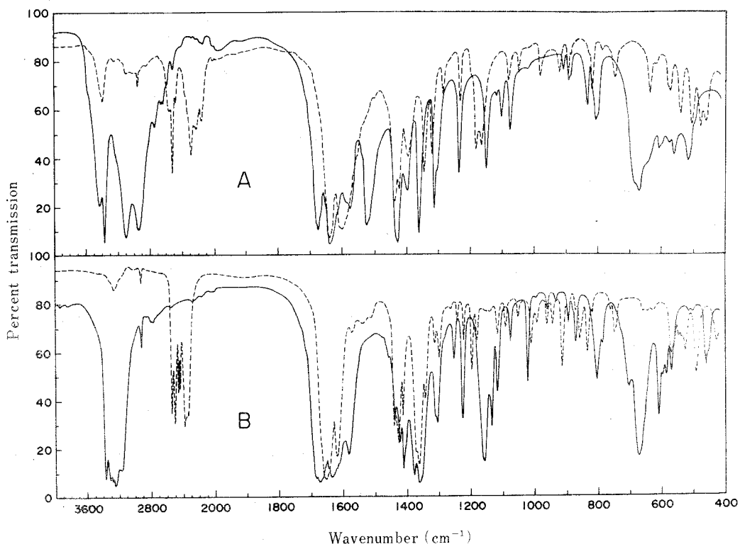
Fig. 1. IR Spectra of \text{Asn} \cdot \text{H}_2\text{O} and [\text{Cu}(\text{asn})_2]_n in the Region above 400\text{ cm}^{-1}
