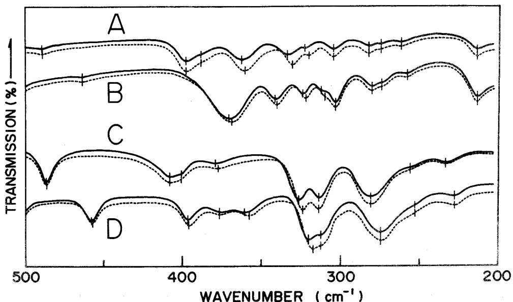
Fig. 3 Expanded IR Spectra of t -Cu(ala) _2 , t -Cu(ala- d_2 ) _2 , c -Cu(ala) _2 and c -Cu(ala- d_2 ) _2 in the Region between 500 and 200 \text{cm}^{-1} , A : t - ^{63}\text{Cu} (ala) _2 (—) and t - ^{65}\text{Cu} (ala) _2 (----); B : t - ^{63}\text{Cu} (ala- d_2 ) _2 (—) and t - ^{65}\text{Cu} (ala- d_2 ) _2 (----); C : c - ^{63}\text{Cu} (ala) _2 (—) and c - ^{65}\text{Cu} (ala) _2 (----); D : c - ^{63}\text{Cu} (ala- d_2 ) _2 (—) and c - ^{65}\text{Cu} (ala- d_2 ) _2 (----).
