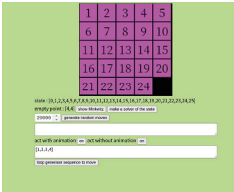
24-puzzle
