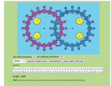
hungarian rings
