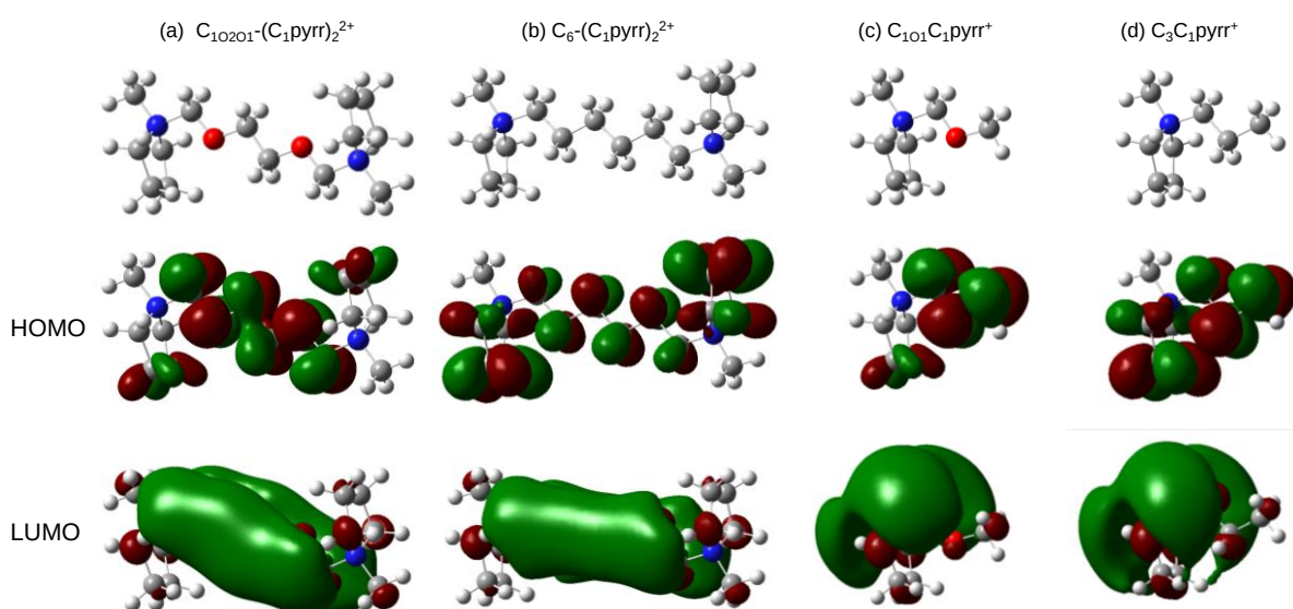
Figure 7 The HOMO and LUMO diagrams of (a) C_{10201}-(C_1pyrr)_2^{2+} , (b) C_6-(C_1pyrr)_2^{2+} , (c) C_{101}C_1pyrr^+ , and (d) C_3C_1pyrr^+ at the 0.02 e bohr -3 isosurfaces.
