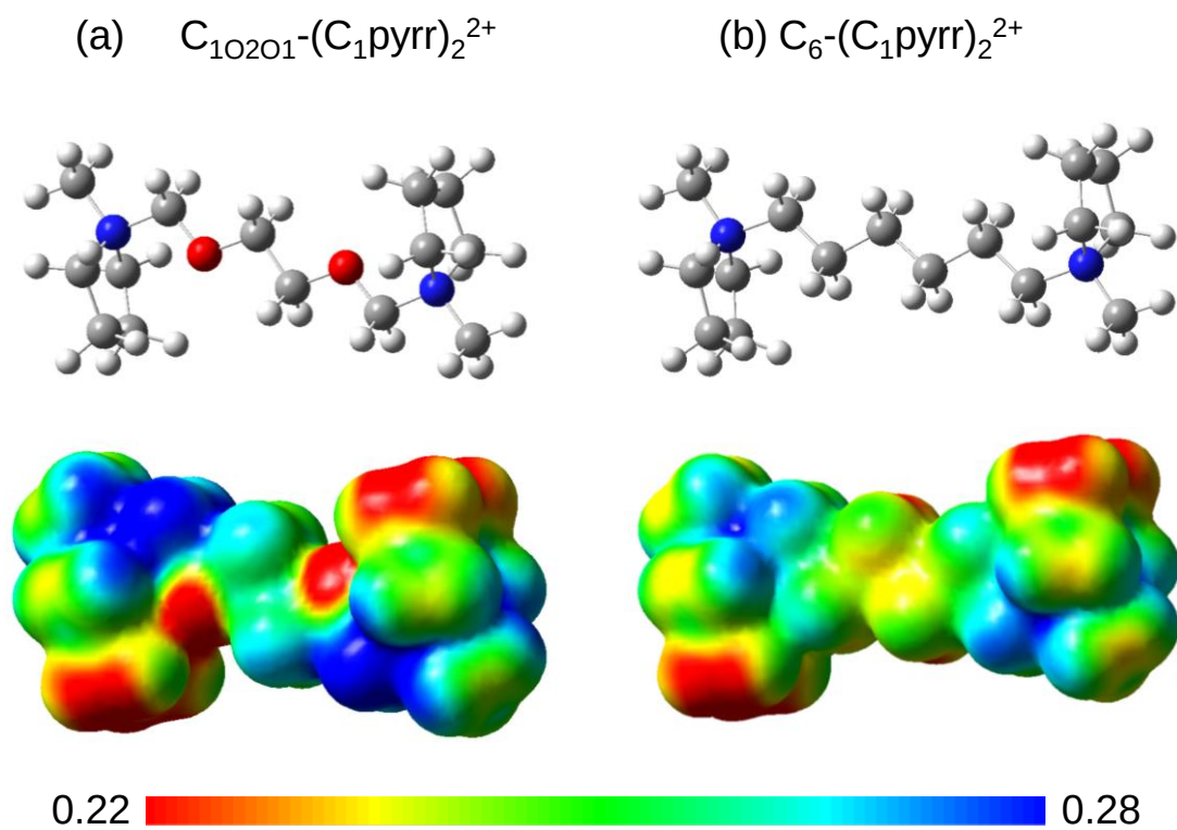
Figure 2 Optimized structures and electrostatic potential maps at the 0.005 \text{ e bohr}^{-3} isosurfaces of (a) C_{10}O_2O_1-(C_1pyrr)_2^{2+} and C_6-(C_1pyrr)_2^{2+} .
