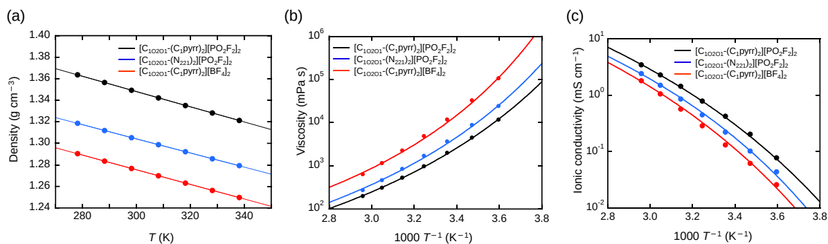
Figure 4 Temperature dependence of (a) densities, (b) viscosities, and (c) ionic conductivities for [\text{C}_{10201}-(\text{C}_1\text{pyrr})_2][\text{PO}_2\text{F}_2]_2 , [\text{C}_{10201}-(\text{N}_{221})_2][\text{PO}_2\text{F}_2]_2 , and [\text{C}_{10201}-(\text{C}_1\text{pyrr})_2][\text{BF}_4]_2 (see Tables S1, S2, and S3 for the data of density, viscosity, and ionic conductivity).
