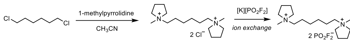
Scheme 2 The synthetic route of the [\text{C}_6\text{-(C}_1\text{pyrr)}_2][\text{PO}_2\text{F}_2]_2 DIL.
