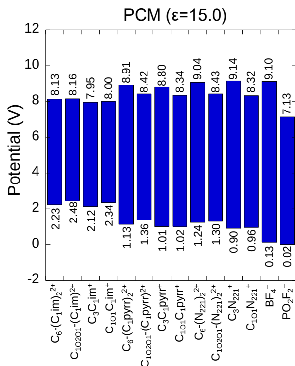
Figure 6 Electrochemical stabilities of the dications, monocations, and anions in this study calculated at the PBE1PBE/aug-cc-pVDZ level using the PCM model with a dielectric constant of 15. See Figure S1 for the structures of the chemical speices and Figure S4 for the electrochemical stabilities under vacuum.
