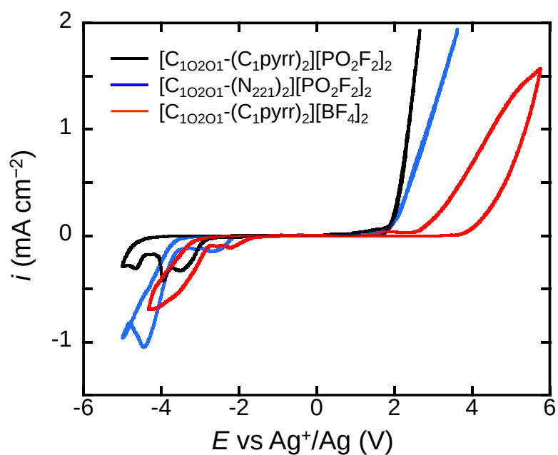
Figure 5 Cyclic voltammograms of a glass-like carbon electrode in [C_{10201}-(C_1pyrr)_2][PO_2F_2]_2 , [C_{10201}-(N_{221})_2][PO_2F_2]_2 , and [C_{10201}-(C_1pyrr)_2][BF_4]_2 . Scan rate: 5 \text{ mV s}^{-1} .
