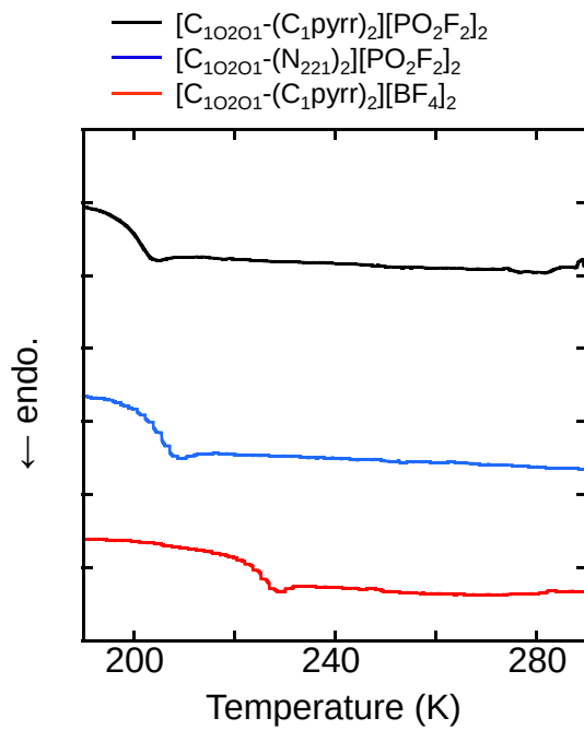
Figure 3 DSC curves of [\text{C}_{10}\text{Z01}-(\text{C}_1\text{pyrr})_2][\text{PO}_2\text{F}_2]_2 , [\text{C}_{10}\text{Z01}-(\text{N}_{221})_2][\text{PO}_2\text{F}_2]_2 , and [\text{C}_{10}\text{Z01}-(\text{C}_1\text{pyrr})_2][\text{BF}_4]_2 under Ar atmosphere. Scan rate: 5 \text{ K min}^{-1} .
