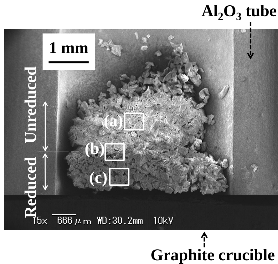
Fig. 4 SEM image of the cross section of the working electrode after electrolysis at 0.5 V vs. \text{Ca}^{2+}/\text{Ca} for 10 min in molten \text{CaCl}_2 at 1123 K. \text{SiO}_2 size: 0.10–0.25
