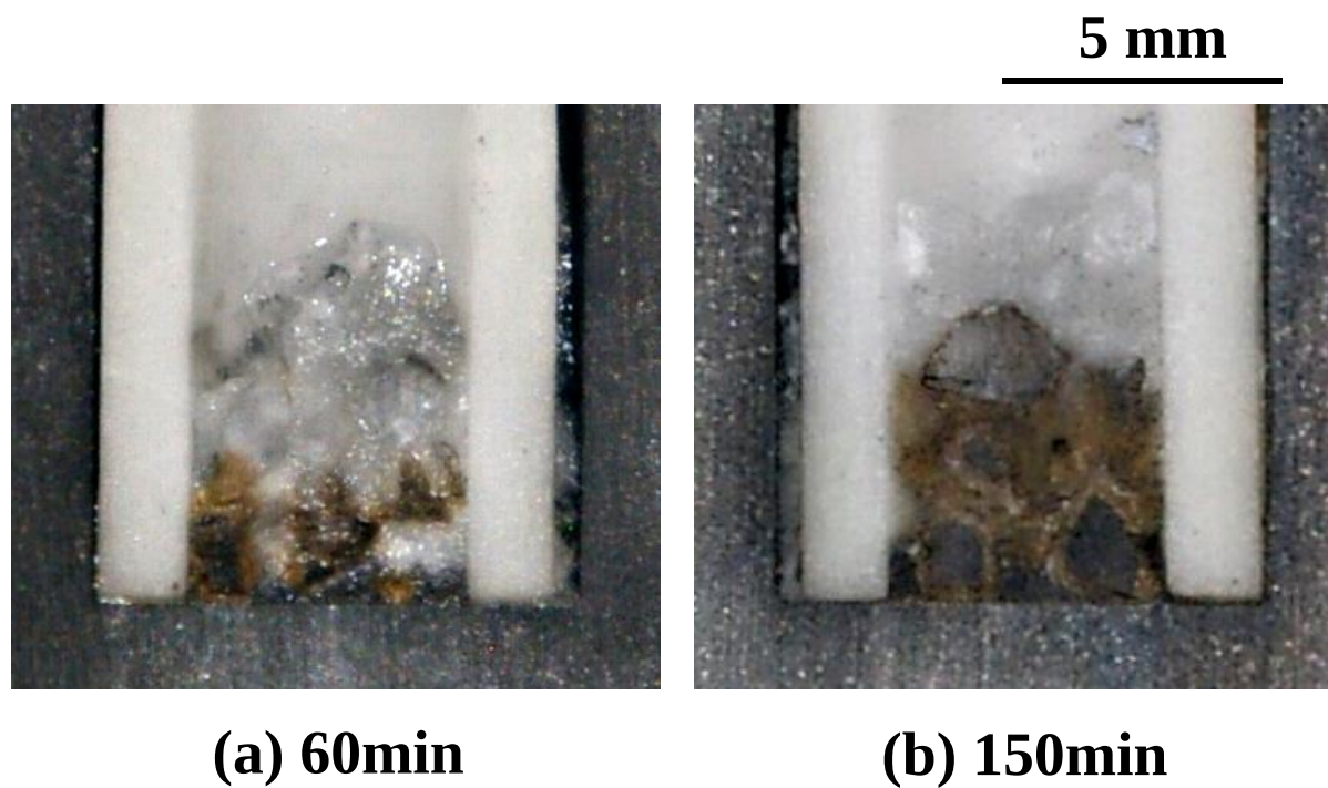
Fig. 6 Photographs of the cross sections of the working electrodes after electrolysis at 0.5 V vs. \text{Ca}^{2+}/\text{Ca} for 60 min and 150 min in molten \text{CaCl}_2 at 1123 K. \text{SiO}_2 size: 1.0–2.0 mm.
