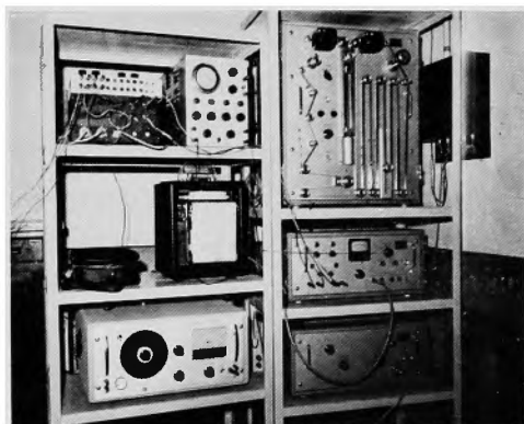
Fig. 6(b). Correlator on right and filter, recorder, and oscillator on left, up to down.
