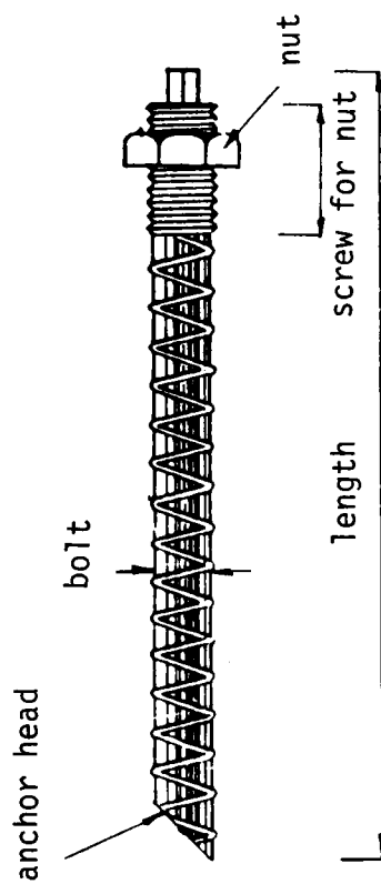
Fig. 9.3 Top-Bonded-Type Rockbolt
