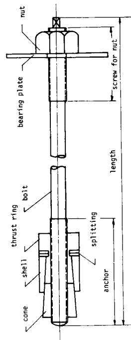
Fig. 9.2 Expansion-Type Rockbolt
