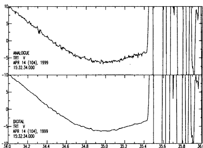
Fig. 11 Magnified portion of the waveform shown in Fig.9. High frequency noise is observed in the waveform obtained from the old system.
