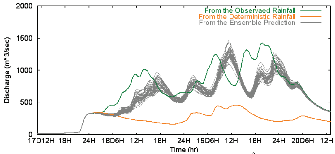
(b) Discharge hydrographs at Ieno (476 km²)
