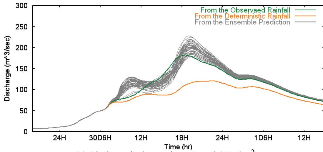
(a) Discharge hydrographs at Ootori (156 km²)
