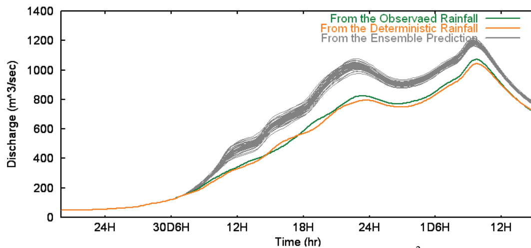
(c) Discharge hydrographs at Kamo (1469 km²)
