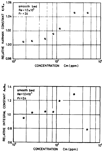
Fig. 22. Relation of Kármán constant or integral constant and mean concentration.
