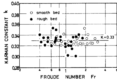
Fig. 13 Effect of Froude number on the Kármán constants.
