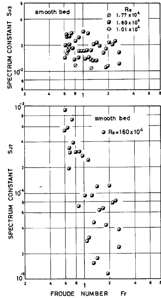
Fig. 2. Effect of Froude number on spectral constants in viscos subrange.
