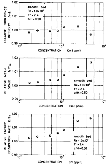
Fig. 23. Relation of turbulence intensity, mean scale or turbulent energy dissipation rate and mean concentration.
