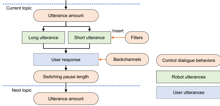
Figure 3. The proposed method of controlling dialogue behaviors for character expression
