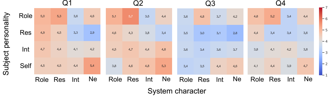
Figure 6. Mean evaluation scores (7-point scales) in each combination of system character and subject personality in laboratory guide. Role: Role model, Res: Reserved, Int: Introvert, Self: Self-centered, Ne: Neutral
