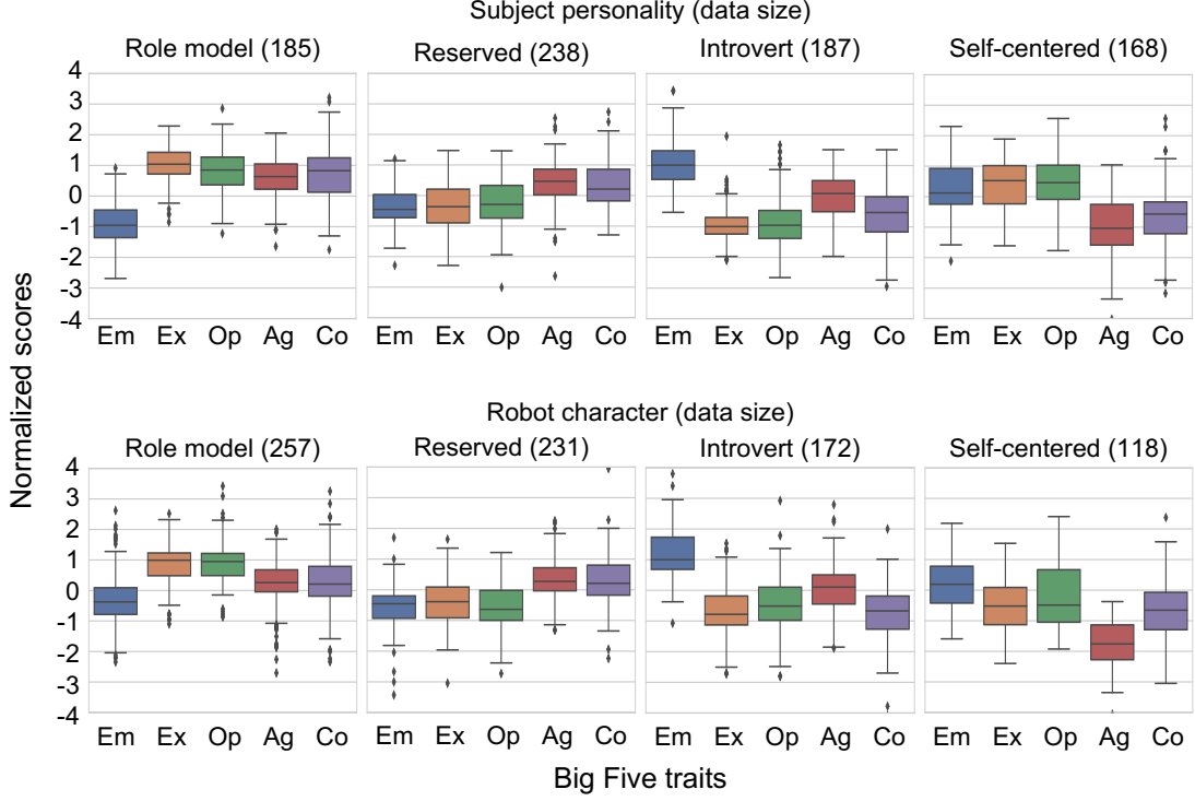
Figure 2. Classification results of Big Five traits on the subject personality and the robot (WOZ) character in corpus
