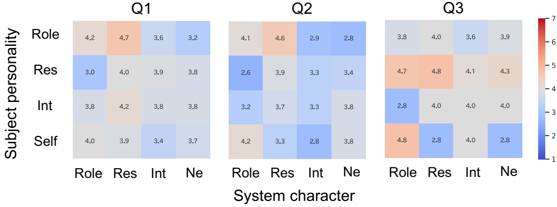
Figure 8. Mean evaluation scores (7-point scales) in each combination of system character and subject personality in chit-chat. Role: Role model, Res: Reserved, Int: Introvert, Self:Self-centered, Ne: Neutral
