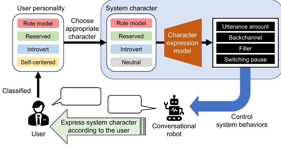
Figure 1. An overview of the character expression method
