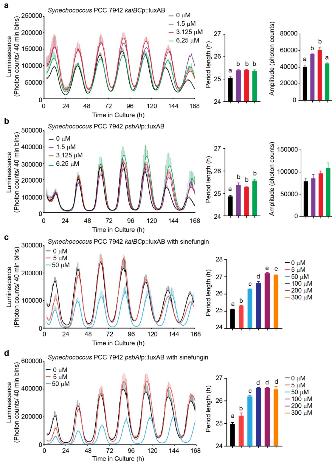
Figure 5. The link between the methyl cycle and the clock is conserved in cyanobacteria. (a) Left panel shows mean luminescence \pm SEM of Synechococcus PCC 7942 kaiBCp::luxAB knock-in strain treated with different concentrations of DZnep, n = 3 , with only the upper section of the error bars shown for clarity. Middle panel shows mean period \pm SEM, n = 3 . Right panel shows mean amplitude \pm SEM, n = 3 . (b) Same as (a) but using Synechococcus PCC 7942 psbAip::luxAB knock-in
