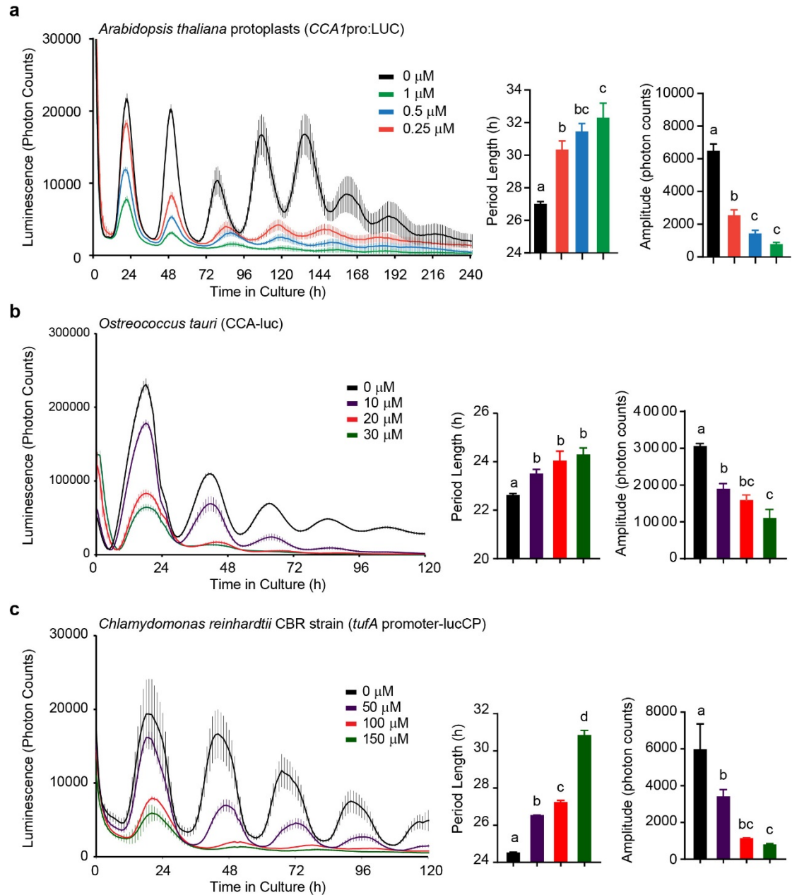
Figure 4. The link between the methyl cycle and the clock is conserved in plants. (a) Left panel shows mean luminescence \pm SEM of Arabidopsis thaliana protoplasts bearing a CCA1pro:LUC reporter construct, n = 8 wells per treatment, treated with different concentration of DZnep. For comparison between different runs, traces were aligned in relation to the first peak. Middle panel shows mean \pm SEM of amplitude, n = 8 . Right panel shows mean \pm SEM of amplitude, n = 8 . (b) Same as (a) but with Ostreococcus tauri cells carrying a CCA1-LUC reporter, n = 8 wells. Middle panel shows mean \pm SEM of period, n = 8 wells. No significance was observed between 10, 20 and 30 \mu M, but the significance compared to 0 \mu M became stronger, i.e. p < 0.05 , p < 0.001 , p < 0.0001 , respectively, indicating dose-dependent effects. Right panel shows mean \pm SEM of amplitude, n = 8 wells. (c) Same as (b)
