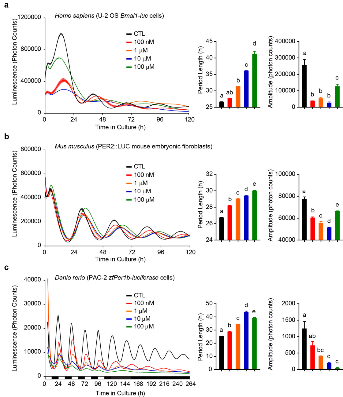
Figure 2. The link between the methyl cycle and the clock is conserved in vertebrates. (a) Left panel shows mean luminescence \pm SEM of human U2OS cells stably transfected by a Bmal1-luc reporter and treated with increasing concentrations of DZnep. Middle panel shows mean \pm SEM of period, n = 3 . Right panel shows mean \pm SEM of amplitude, n = 3 dishes. Same analyses were performed with PER2::LUC mouse embryonic fibroblasts, n = 3 dishes (b), and PAC-2 zebrafish cells stably transfected with a Per1b-luciferase reporter, n = 4 dishes, mean \pm SEM (c). These experiments were independently reproduced at least three times. All bar graphs analyzed by One-Way ANOVA followed by Bonferroni post-hoc test; a vs. b vs. c vs. d vs. e , indicating at least p < 0.05 significance.
