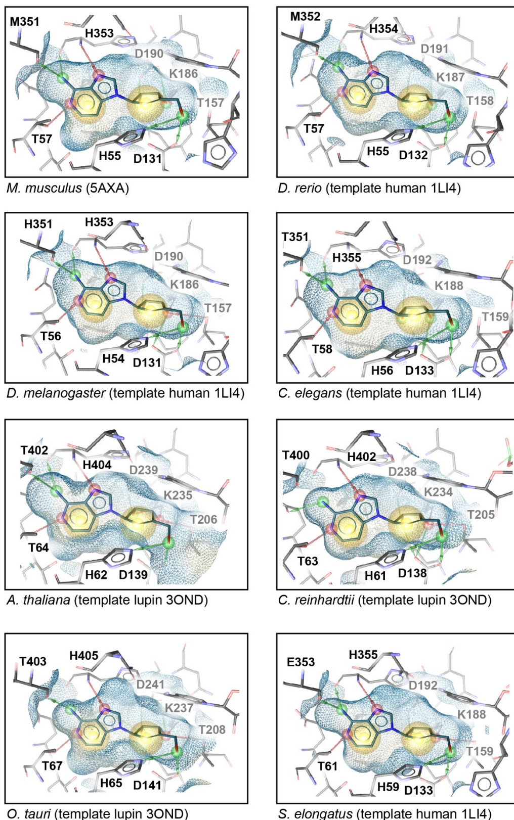
Figure S2. Molecular docking simulations of AHCY with DZnep, related to Fig. 1.
