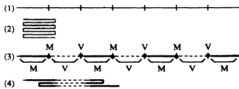
Figure 2: Mountain folding by zig-zag method
