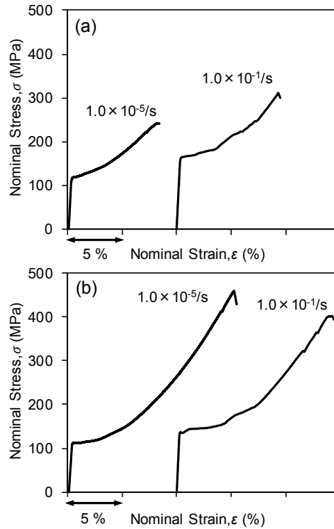
Figure 2. Stress–strain curves of \text{SrTiO}_3 single crystals with different chemical compositions, deformed at constant strain rates of \dot{\epsilon} = 1.0 \times 10^{-5} \text{ (s}^{-1}\text{)} and \dot{\epsilon} = 1.0 \times 10^{-1} \text{ (s}^{-1}\text{)} . (a) \text{Sr}/\text{Ti} = 1.00 , (b) \text{Sr}/\text{Ti} = 1.04 as the starting powders.
