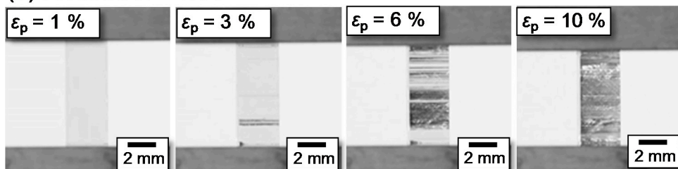
Figure 3. Shapes and surface morphologies of the deformed specimens. (a) The \text{Sr}/\text{Ti} = 1.00 specimen deformed at \dot{\epsilon} = 1.0 \times 10^{-1} \text{ (s}^{-1}\text{)} . (b) The \text{Sr}/\text{Ti} = 1.04 specimen deformed at \dot{\epsilon} = 1.0 \times 10^{-1} \text{ (s}^{-1}\text{)} . Here, each \epsilon_p in the figures indicates the plastic strain.
