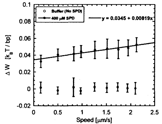
Figure 2: The dependence of \Delta W on the s-r speed at 400 \mu\text{M} SPD (closed circle) and in buffer (open circle).
