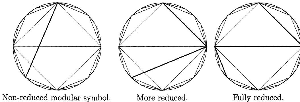
FIGURE 4. The modular symbol \{0, 12/5\} and its reduction in C .
