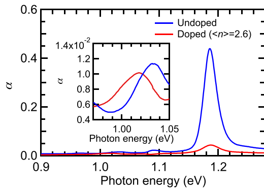
FIG. 1. Optical absorption spectra of undoped and hole-doped single-walled carbon nanotubes. The inset shows an enlarged view of the lower-energy region.
