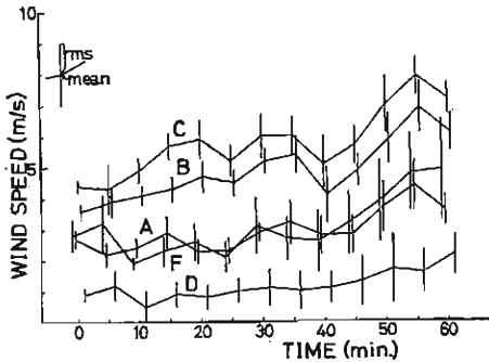
Fig. 5 Changes of mean and rms wind speeds.
