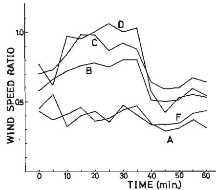
Fig. 4 Ratios of wind speeds to the reference wind speed.
