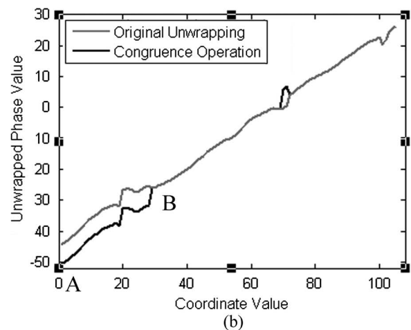
Fig. 4. Comparison between Fig. 1(c) and Fig. 3(e): (a) error map, (b) diagram generated with the 40th row phase data.
