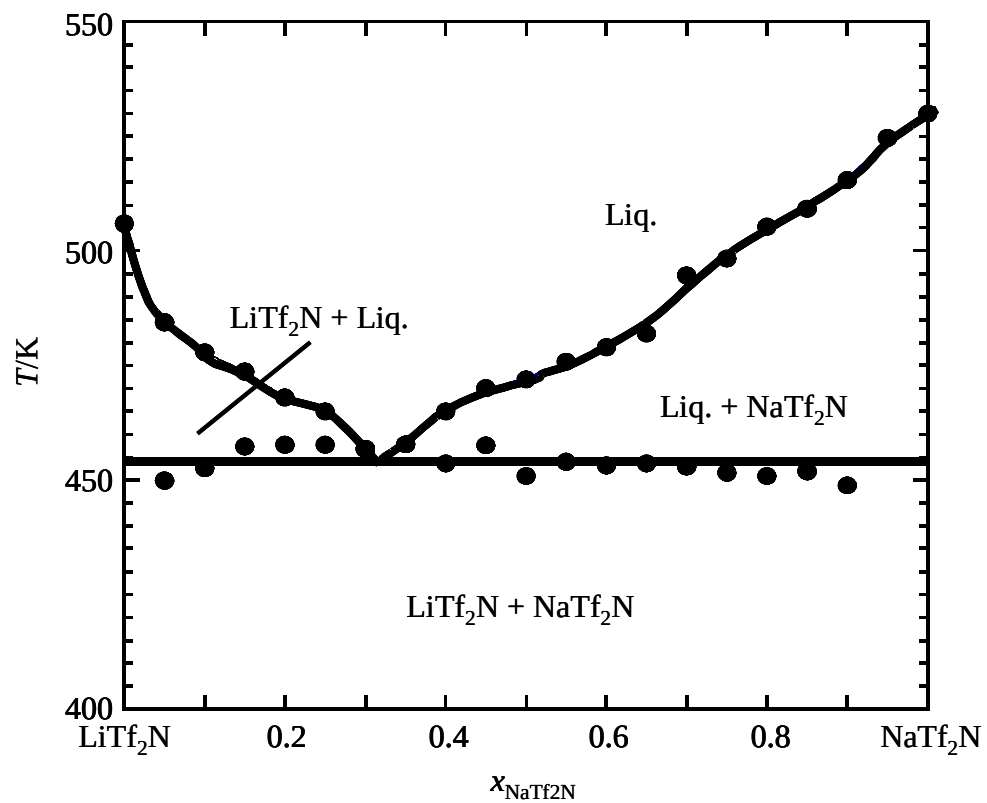
Figure 2. Phase diagram of \text{LiTf}_2\text{N} + \text{NaTf}_2\text{N}
