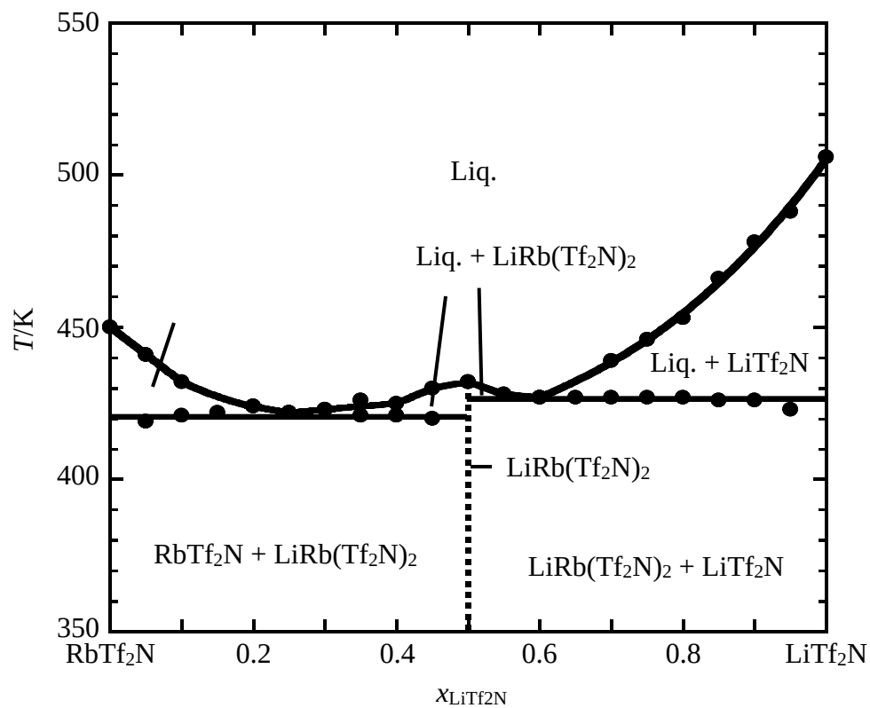
Figure 5. Phase diagram of \text{LiTf}_2\text{N} + \text{RbTf}_2\text{N} .
