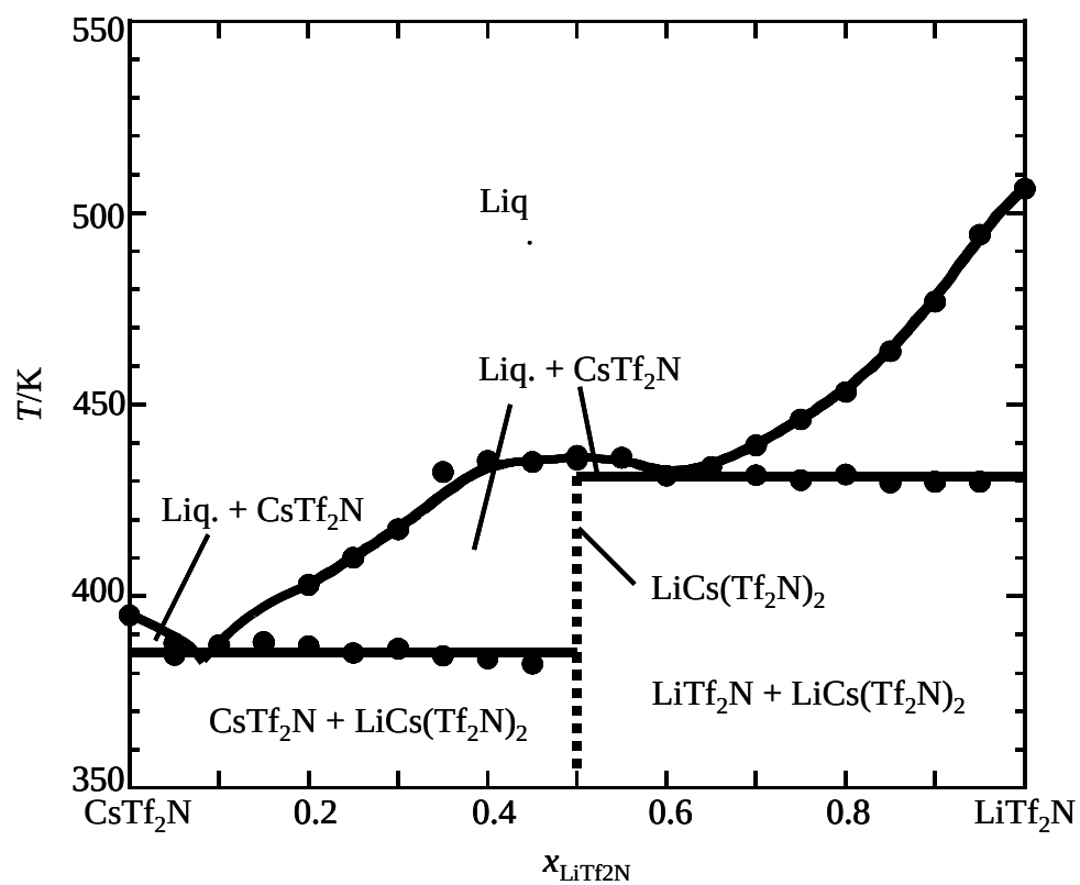
Figure 6. Phase diagram of \text{LiTf}_2\text{N} + \text{CsTf}_2\text{N} .
