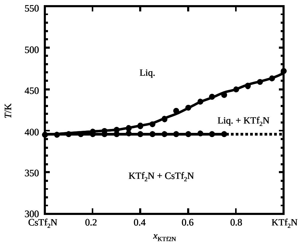
Figure 4. Phase diagram of \text{KTF}_2\text{N} + \text{CsTf}_2\text{N} .
