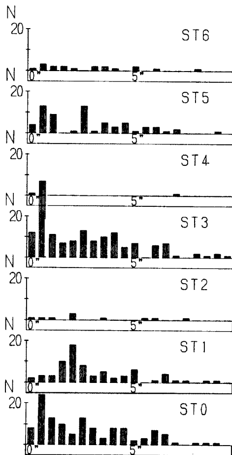
Fig. 10. Frequency distributions of S-P times at all stations.
