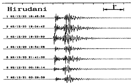
Fig. 9. Examples of earthquakes occurred close to the crater of Mt. Yake-dake volcano recorded at Hirudani (ST3 in Fig. 6).
