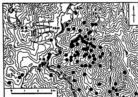
Fig. 2. Epicenter (lower figure) and depth (upper figure) distributions of the earthquake swarm at Kamikochi in September, 1969.
