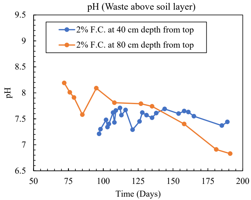
(a) pH for different depths of column with 2% F.C.
