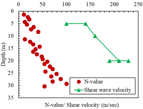
Figure 5.6. Change in N -value and shear wave velocity with depth
