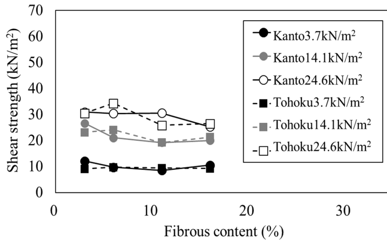
Figure 3.22 Relationship between the content ratio of fibrous materials and shear strength of the waste
