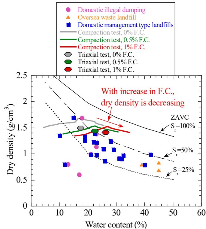
Figure 3.26 Dry density vs water content
