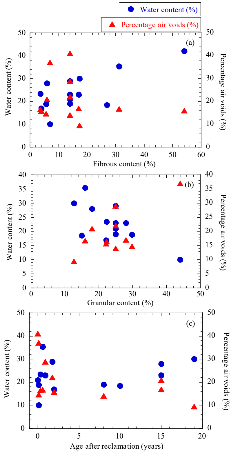
Figure 3.10 Change in water content and percentage air voids for (a) fibrous content, (b) granular content and (c) age after reclamation
