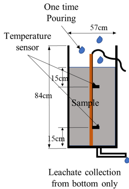
(a) Lysimeter outline
