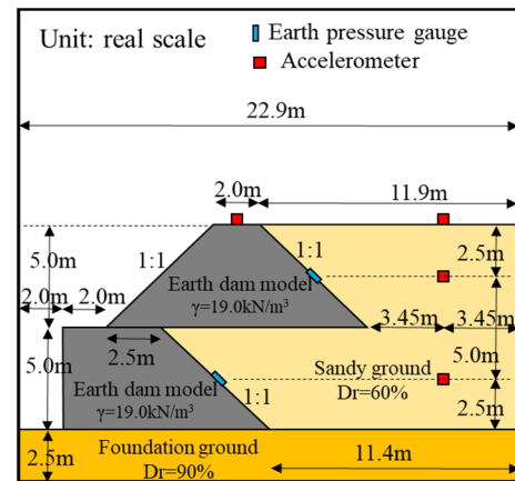
Figure 5.11 Model used for centrifuge test
