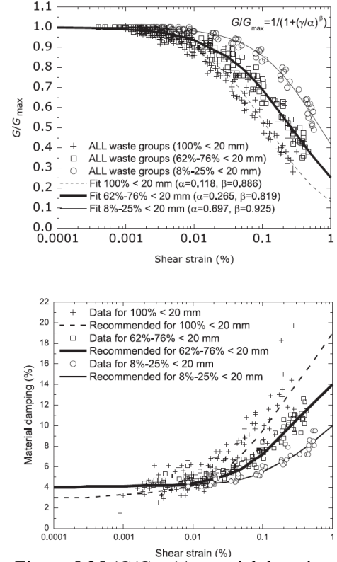
Figure 5.25 (G/G_{max}) / material damping vs shear strain for waste (Zekkos et al. 2008)
