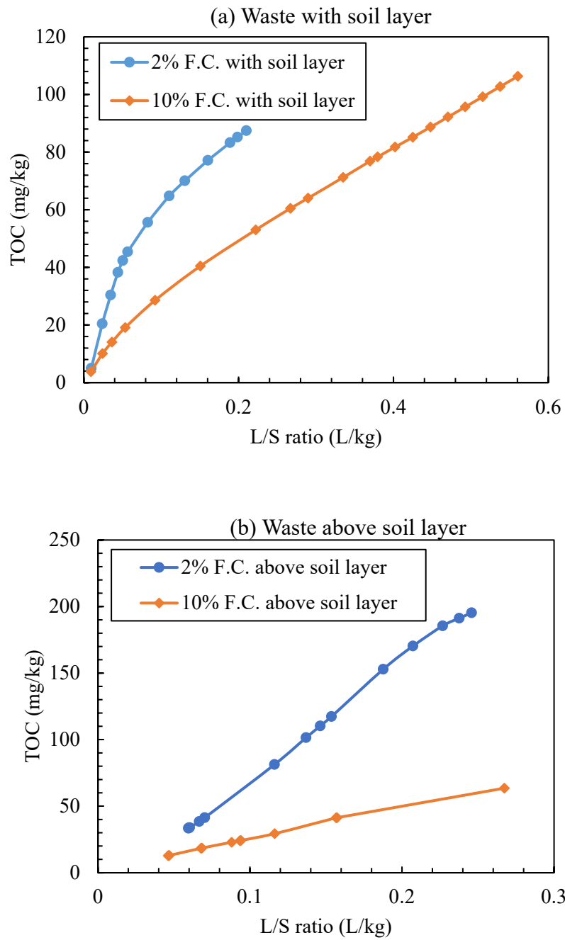
Figure 4.13 Change in TOC with increase in L/S ratio
