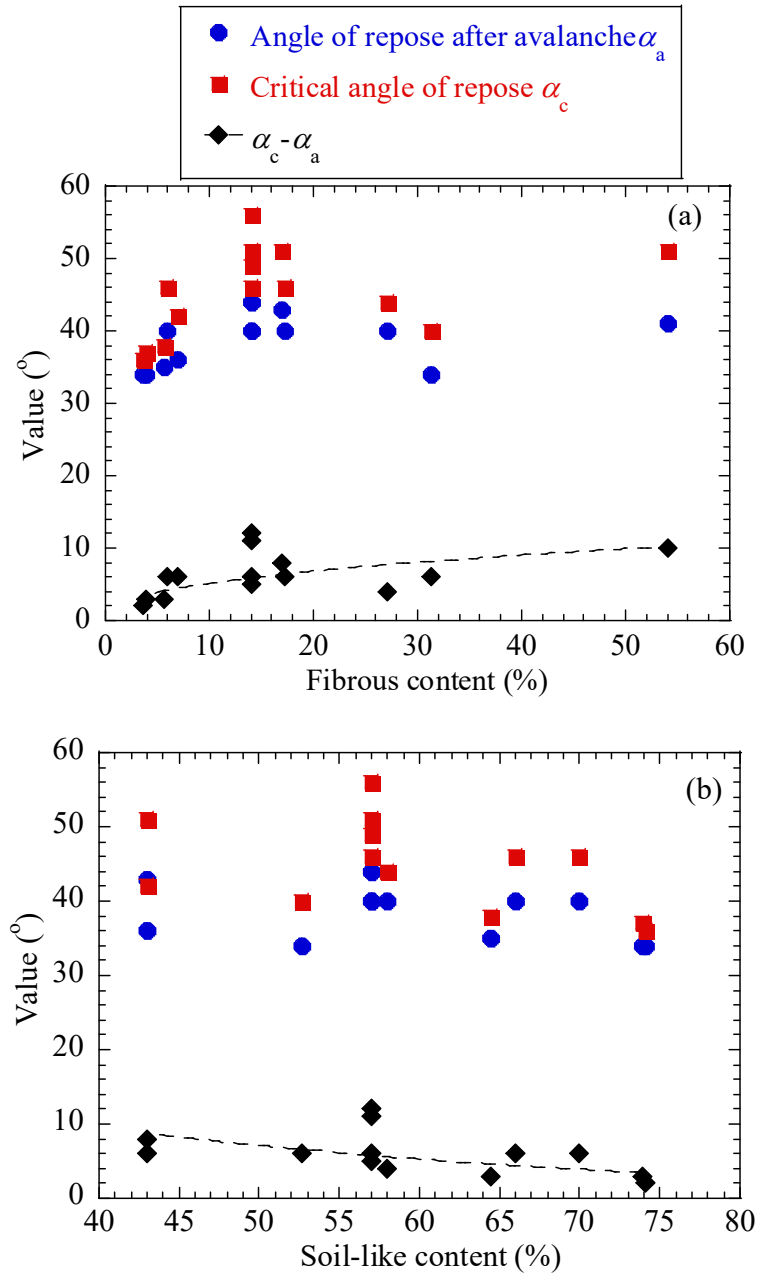
Figure 3.12 Change in critical angle of repose ( \alpha_c ), angle of repose after avalanche ( \alpha_a ), and (\alpha_c - \alpha_a) with (a) fibrous content and (b) soil-like content
