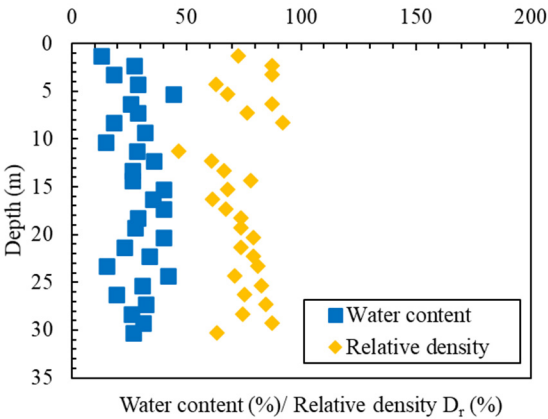
Figure 5.7. Change in water content and relative density with depth
