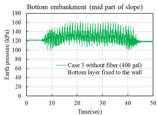
Figure 5.18 Earth pressure at the bottom embankment for case 3 in 200-gal and 400-gal
