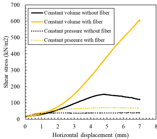
Figure 5.13 Shear stress with increase in horizontal displacement for constant pressure or constant volume
