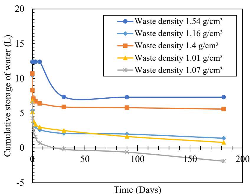
Figure 4.8 Water storage in five cases of lysimeters
