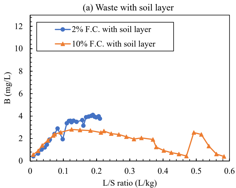
Figure 4.15 Change in boron with increase in L/S ratio
