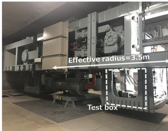
Figure 5.10 Centrifuge machine (Maeda Corporation)
