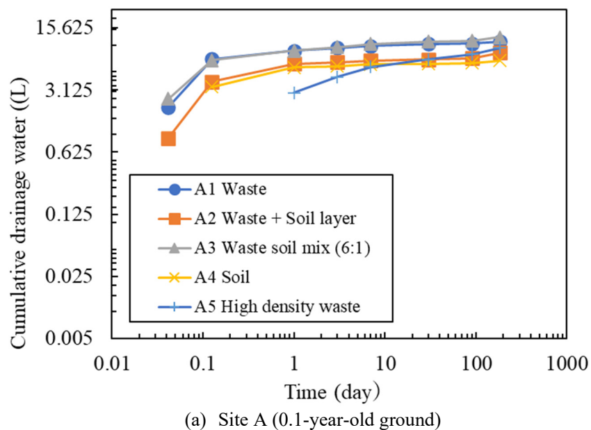
Figure 4.2 Drainage conditions of lysimeters
