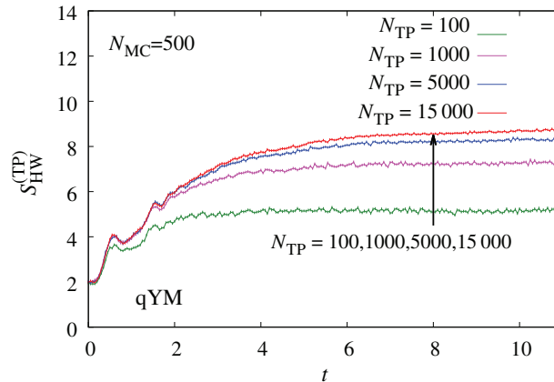
Fig. 1. Time dependence of the HW entropy by using the TP method in qYM, with N_{\text{TP}} = 100, 1000, 5000 , and 15 000, and N_{\text{MC}} = 500 . The arrow shows how the calculated HW entropy changes as N_{\text{TP}} increases.
