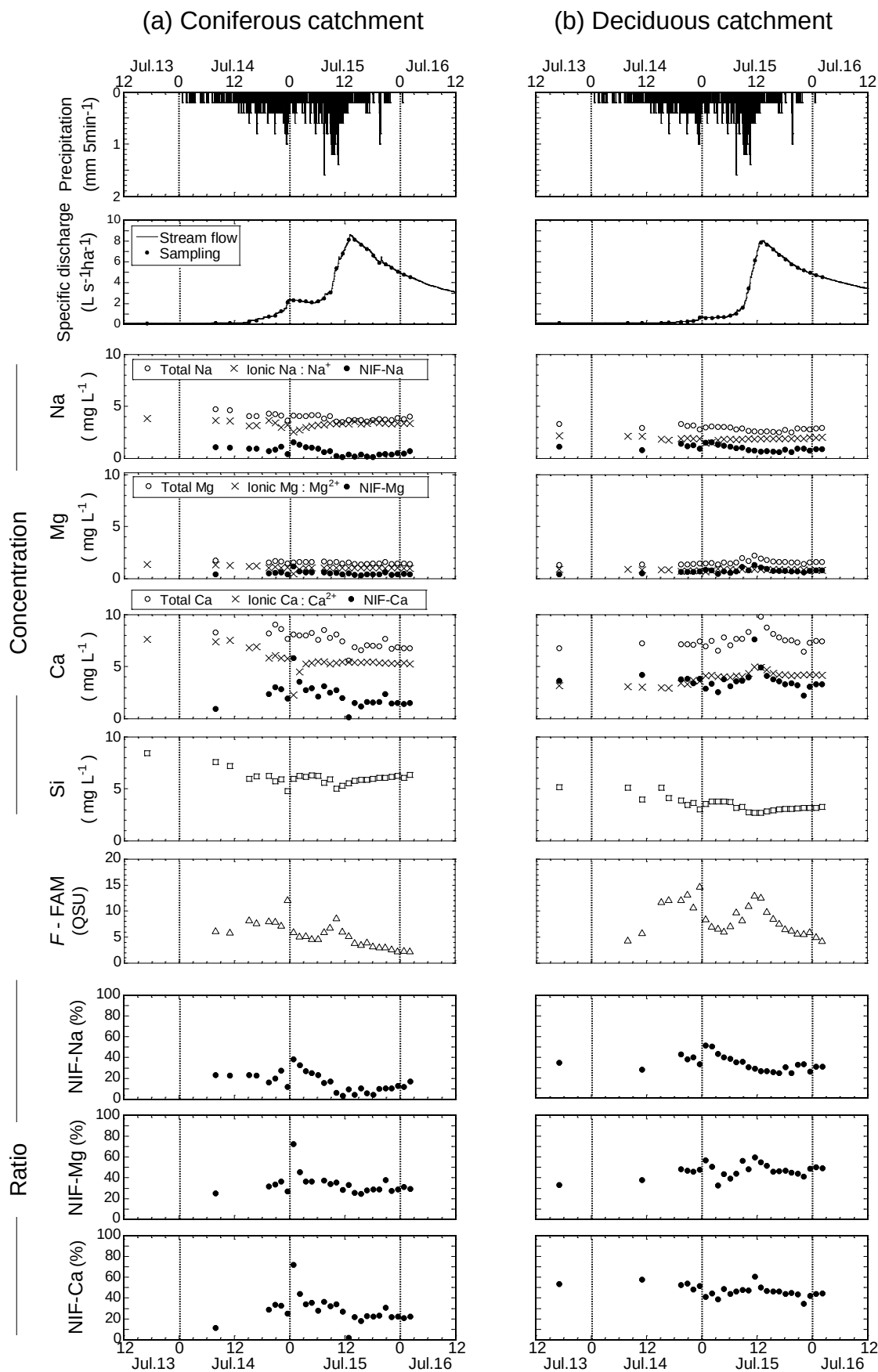
Figure 7. Concentrations of major metals (Na, Mg, and Ca) and silicon (Si), peak fluorescence intensity ( F -FAM), and the proportion of non-free ionic fractions (NIF) relative to total elements in stream water during a typhoon storm in 2007 (Storm 2).
