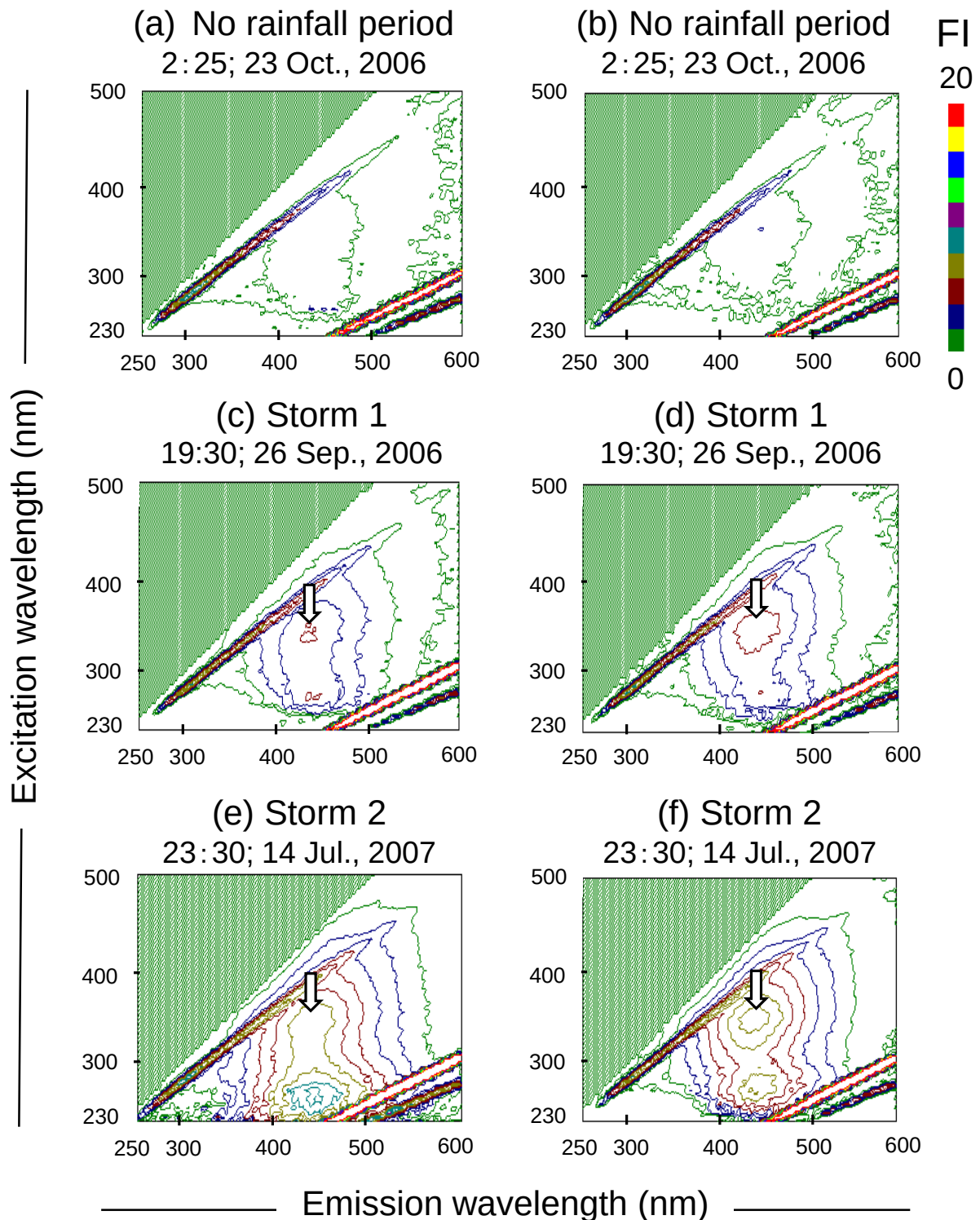
Figure 3 Typical EEM spectra for the different stream flow regimes. The arrows show the visible peaks in fluorescence intensity (FI) at around Ex/Em: 340/440 during the rainstorms. Contour intervals of FI are 1.0.
