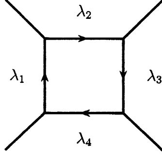
Figure 1: Dual toric diagram of \mathbf{F}_0
