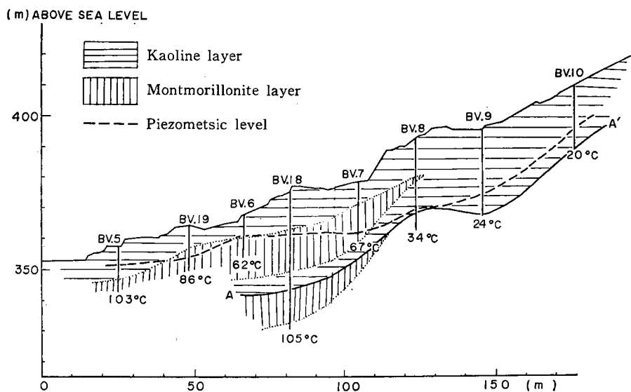
Fig. 2. A sectional distribution of clay minerals along the line C in Fig. 1.
